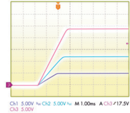
Output powerMod Start-Up
