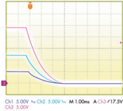
Output powerMod Shutdown
