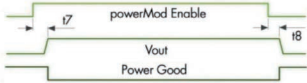
Output powerMod Signals
