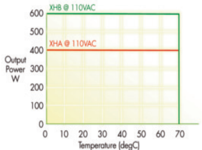
XHA/XHB @ 110VAC Derating
