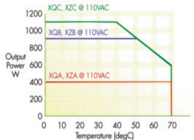
XQA/XQB/XQC and XZA/XZB/XZC @ 110VAC Derating
