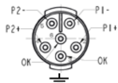
8MF1 P1 and/or P2: 12-48VDC
