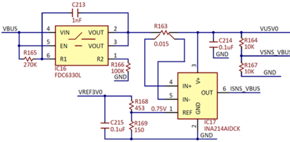
Figure 11 VBUS monitoring. □
