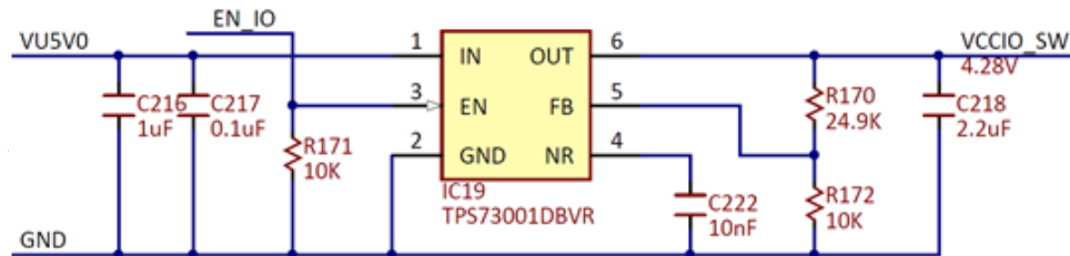
Figure 5. VCCIO_SW supply. []
