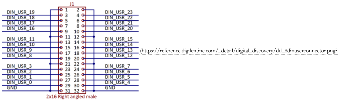
Figure 8. DIN user connector. []
