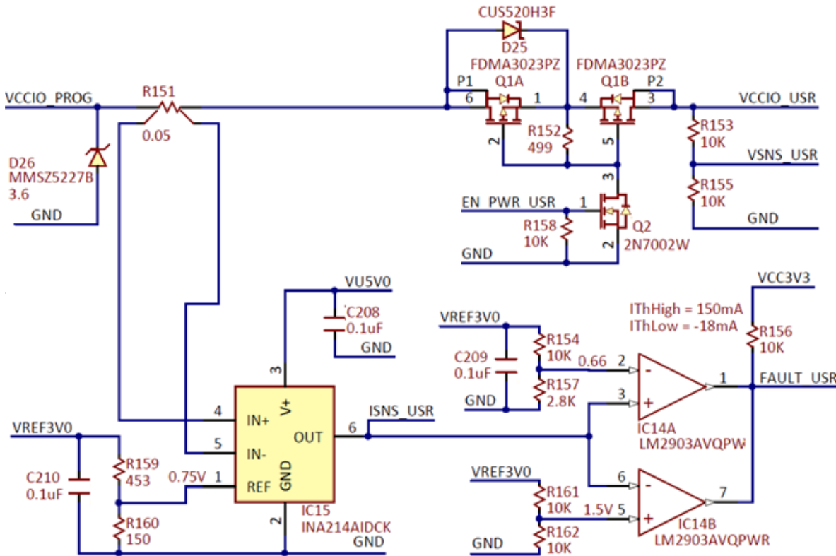
Figure 13. VCCIO_PROG supply. □
