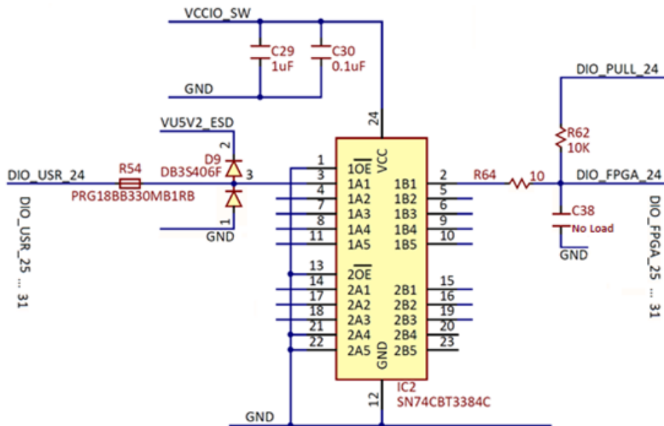
Figure 3. DIO user connectors. []
