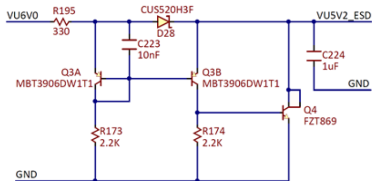
Figure 6. VU6V0 supply. □
