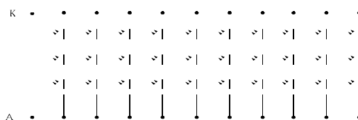
Figure: LED connection of backlight(Constant Current)
