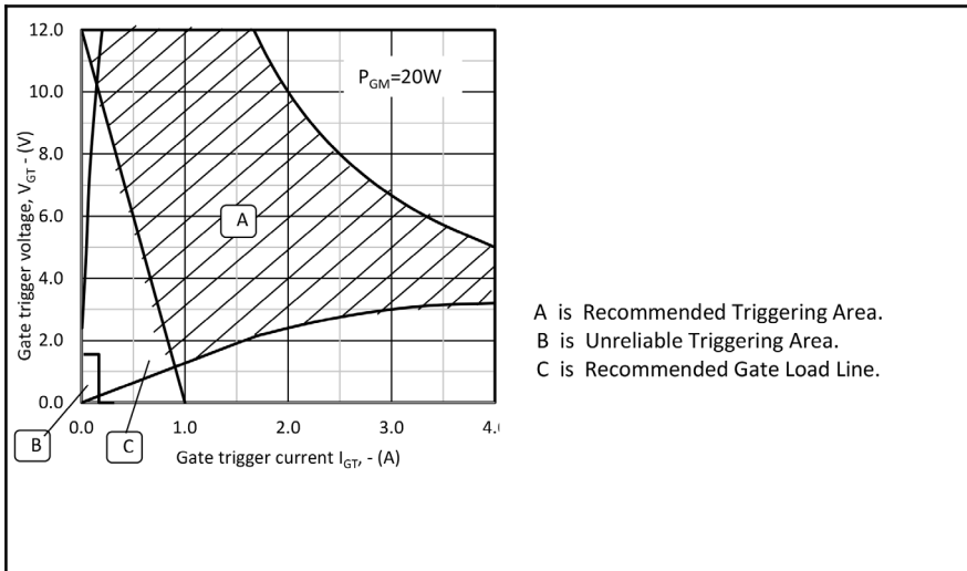
Fig.11 Gate characteristics
