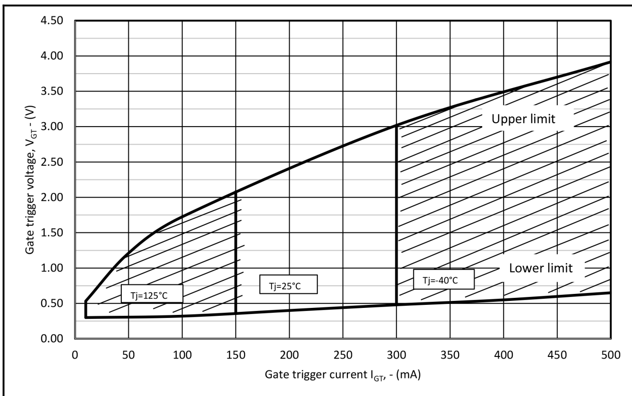
Fig.10 Gate characteristics
