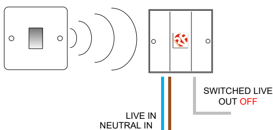
Switch in OFF Position
