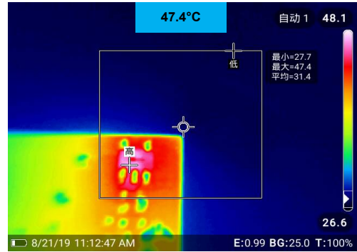
Thermal V_{IN}=265V_{AC}
