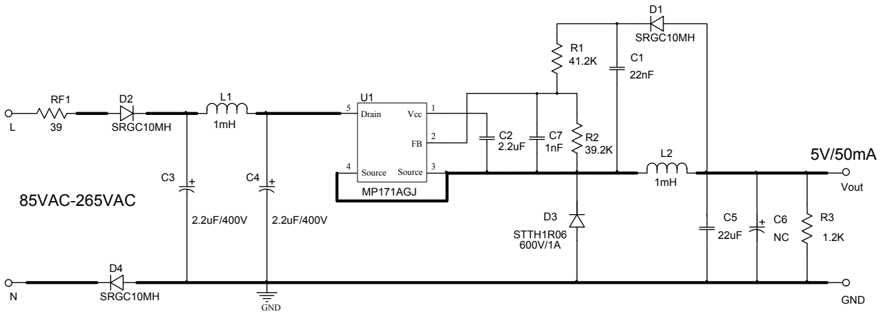
Figure 1: Schematic
