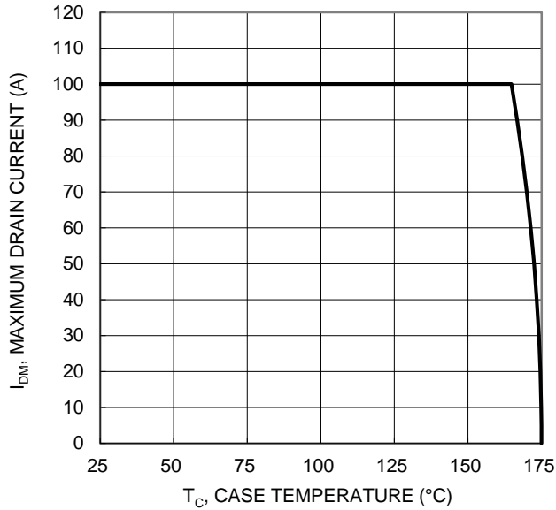
Figure 13. Pulse Current Derating
