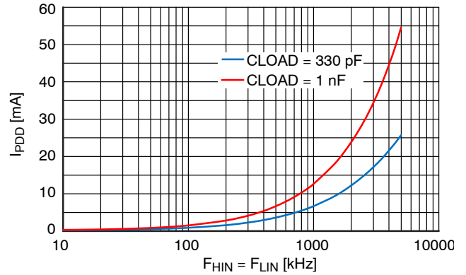
Figure 6. Operating VDD Supply Current ( I_{PDD} ) vs. Frequency (VDD = 12 V, SW = PGND, EN = VDD, Both Outputs Switching)
