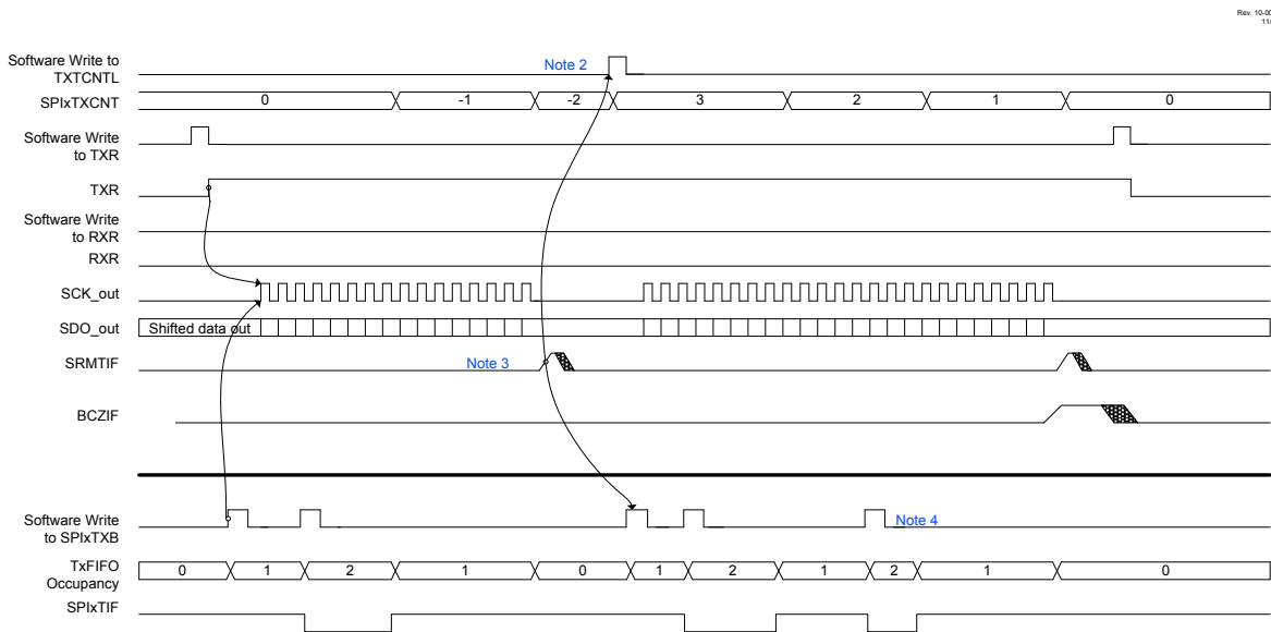
Figure 35-4. SPI Master Operation - Command+Write Data TXR = 1, RXR = 0
