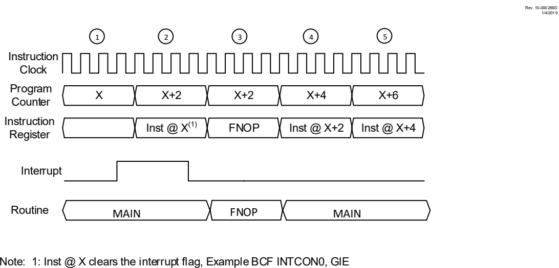
Figure 11-10. Interrupt Timing Diagram: Aborting Interrupts
