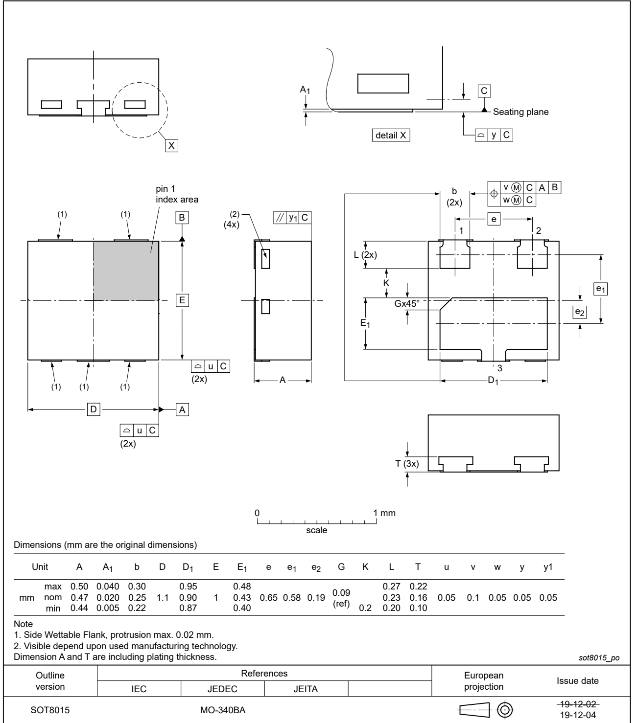
Fig. 12. Package outline DFN1110D-3 (SOT8015)
