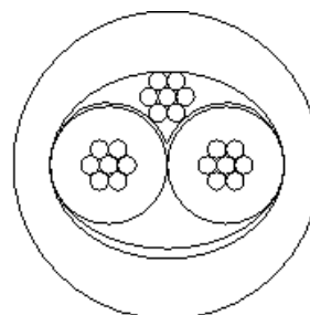
Cable Diagram
