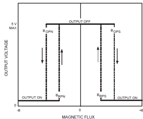
Magnetic Flux
