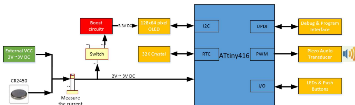
Figure 2-2. Block Diagram of the P4 Board
