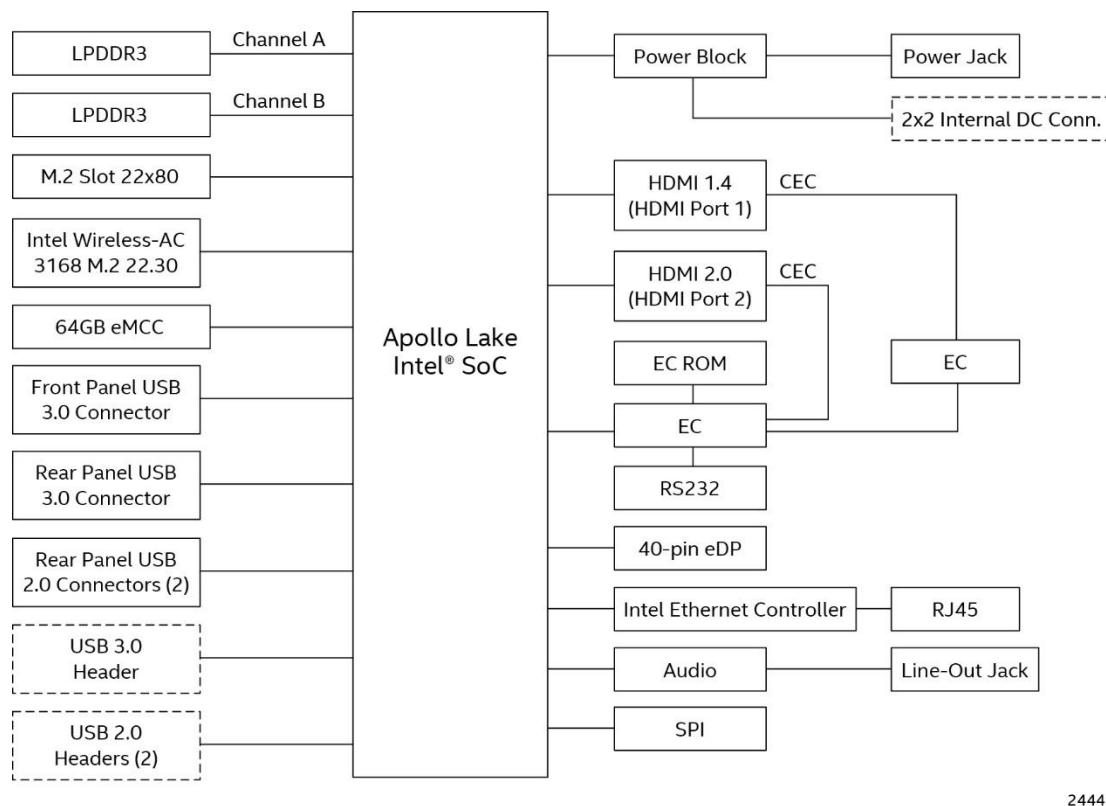
Figure 10. Block Diagram
