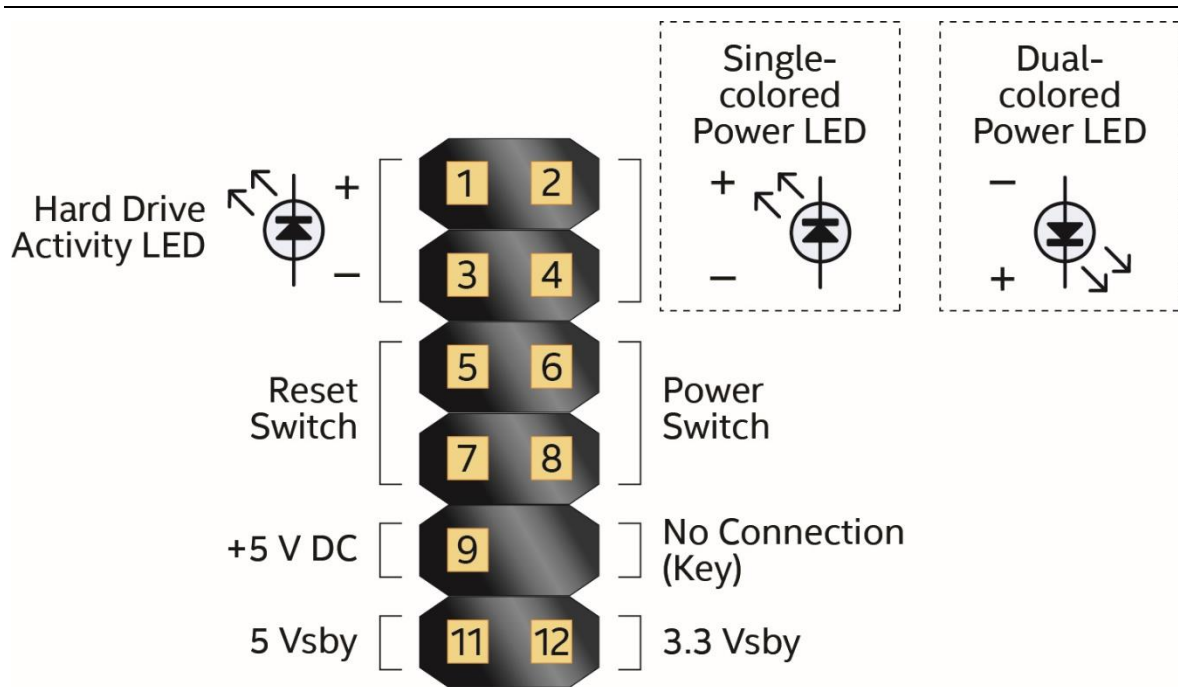
Figure 2. Connection Diagram for Front Panel Header (2.0 mm Pitch)
