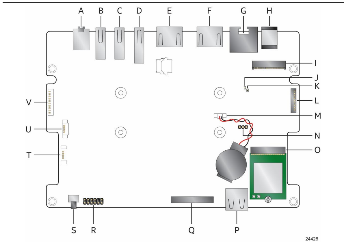
Figure 9. Major Board Components (Bottom)
