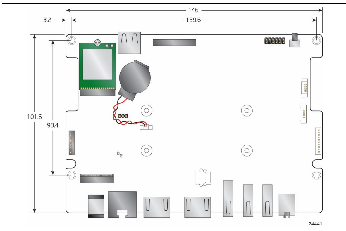
Figure 6. Board Dimensions
