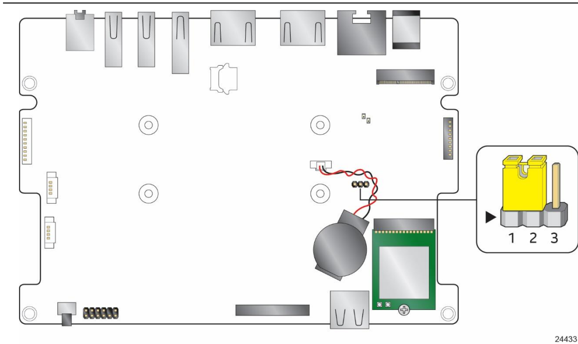
Figure 11. Location of the BIOS Security Jumper
