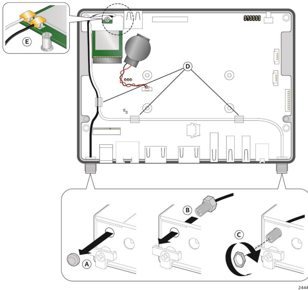
Figure 1. Antenna Wire Routing
