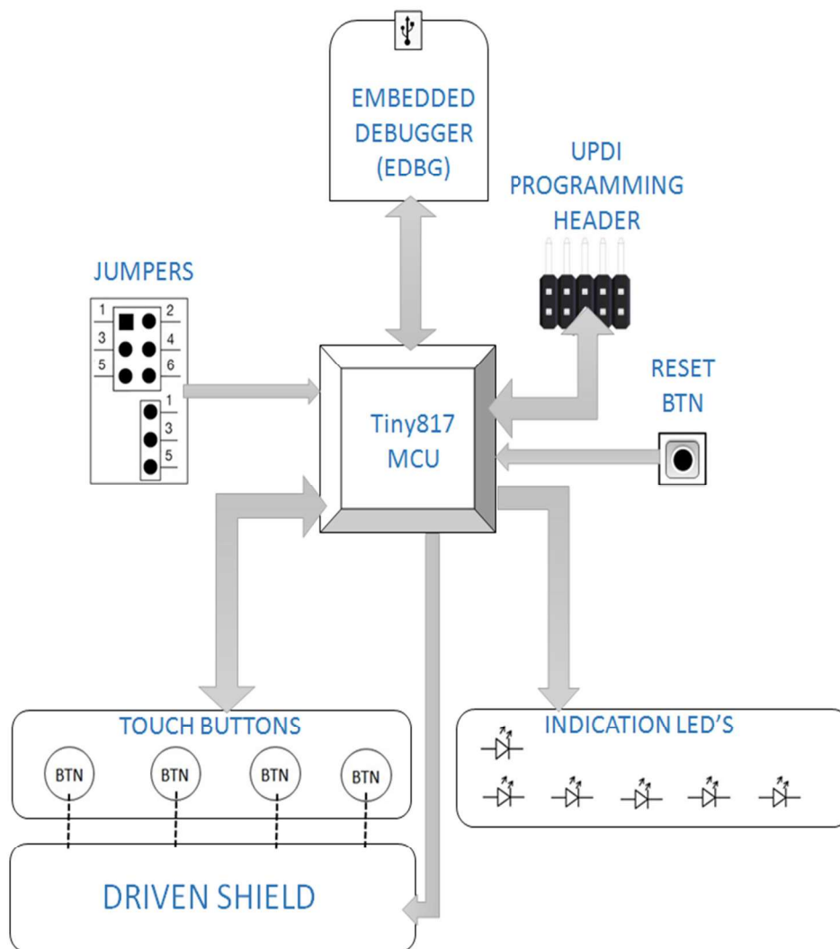
Figure 2-1. Block Diagram
