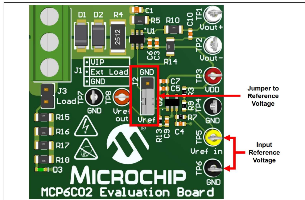
FIGURE 2-4: Using V_{REF} .
