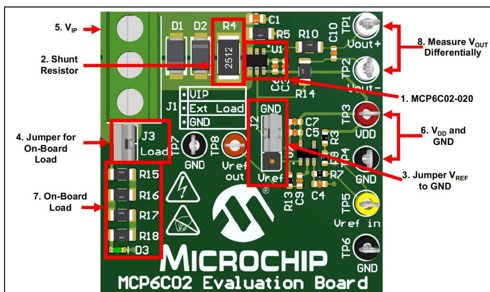
FIGURE 2-3: Out-of-the-Box Setup.
