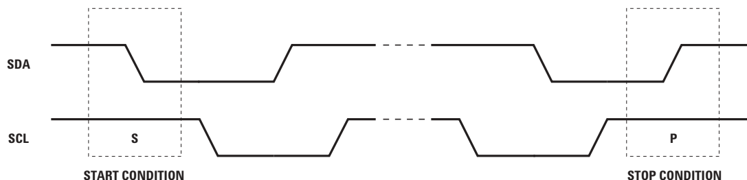
Figure 2. START/STOP condition.
