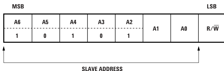
Figure 7. Slave addressing.
