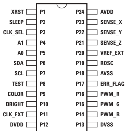
Top View 24-Pin SOIC
