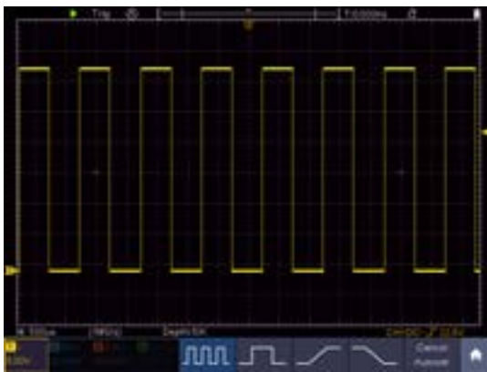
Figure 3-5 Auto set
