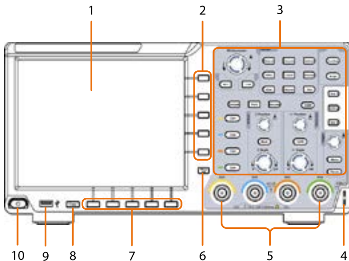
Figure 3-1 Front panel
