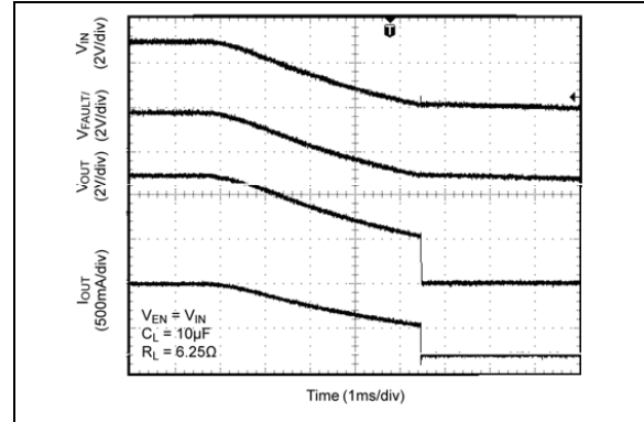
FIGURE 2-28: Turn-Off V IN .
