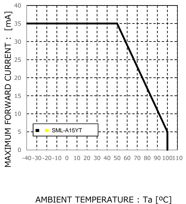
Fig.4 Derating
