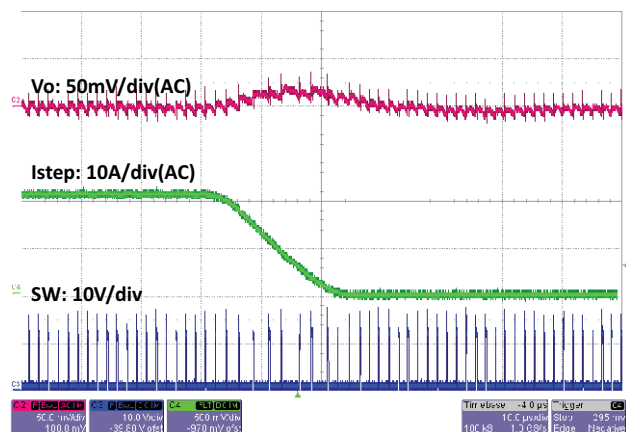
Fig. 54 - SiC450 Load Step, 40 A to 20 A, 10 A/ \mu\text{s} , t = 10\text{ }\mu\text{s/div}
