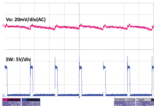
Fig. 41 - SiC451 Output Ripple, 0.01 A, t = 1\text{ }\mu\text{s/div} Forced Continuous Conduction Mode
