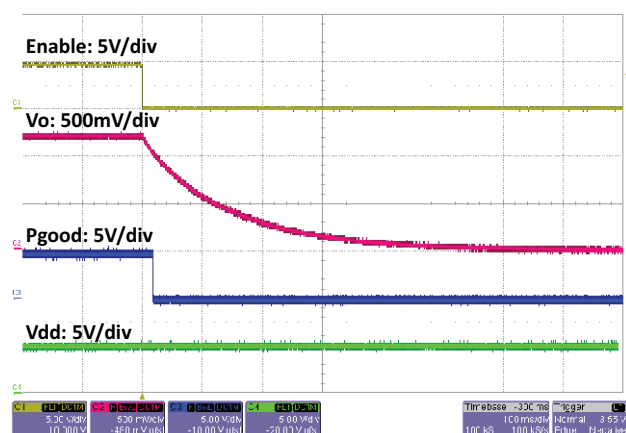
Fig. 50 - SiC450 Shut down with EN, t = 100\text{ ms/div}
