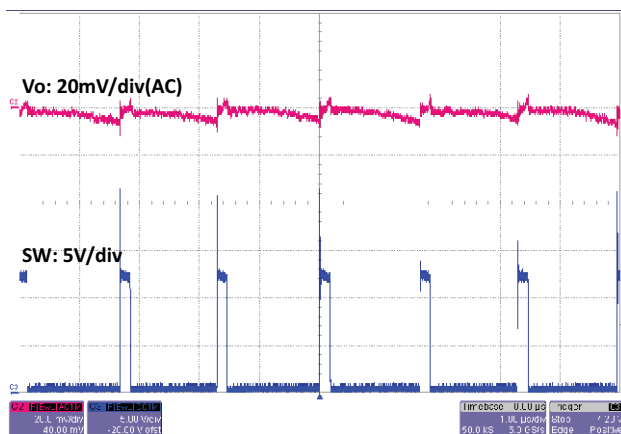
Fig. 43 - SiC451 Output Ripple, 12.5 A, t = 1\text{ }\mu\text{s/div} Forced Continuous Conduction Mode
