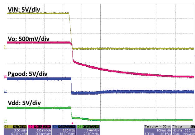
Fig. 48 - SiC450 Shut Down with V_{IN} , t = 100\text{ ms/div}
