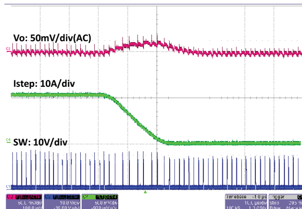
Fig. 56 - SiC450 Load Step, 20 A to 0 A, 1 A/ \mu\text{s} , t = 10\text{ }\mu\text{s/div}
