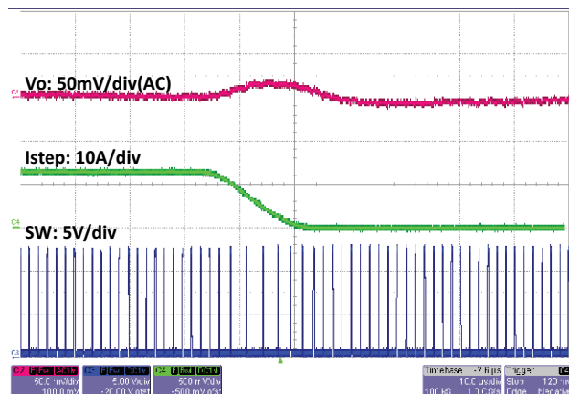
Fig. 38 - SiC451 Load Step, 12.5 A to 0 A, 1 A/μs, t = 10 μs/div
