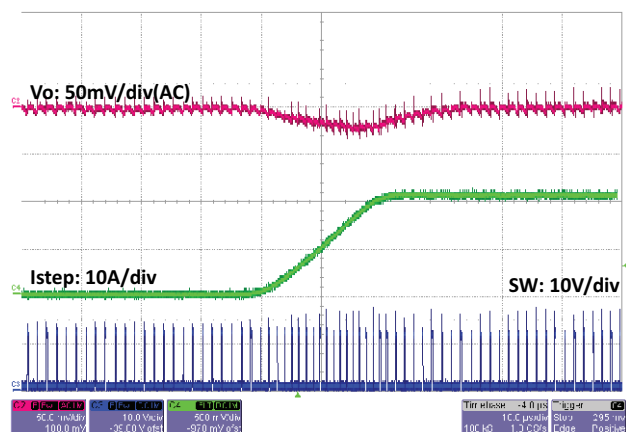
Fig. 55 - SiC450 Load Step, 0 A to 20 A, 1 A/ \mu\text{s} , t = 10\text{ }\mu\text{s/div}
