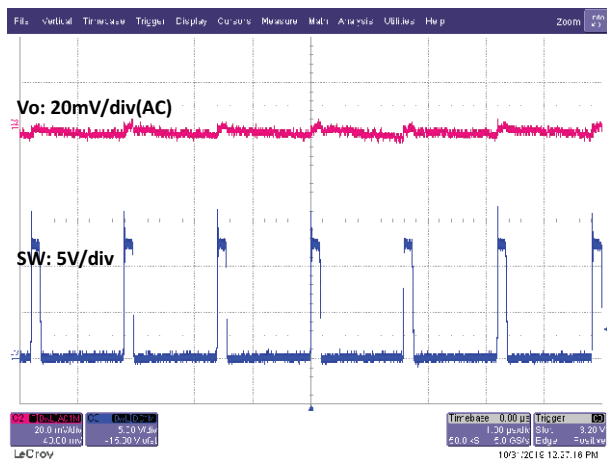
Fig. 59 - SiC450 Output Ripple, 0.01 A, t = 1\text{ }\mu\text{s/div} Forced Continuous Conduction Mode
