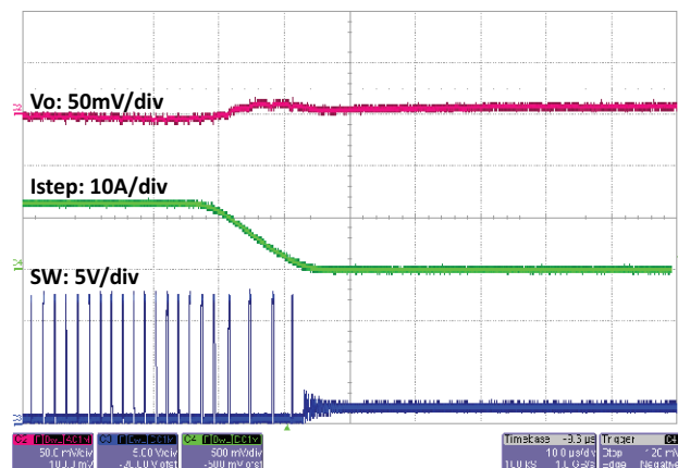
Fig. 40 - SiC451 Load Step, 12.5 A to 0 A, 1 A/μs, t = 10 μs/div Skip Mode Enabled
