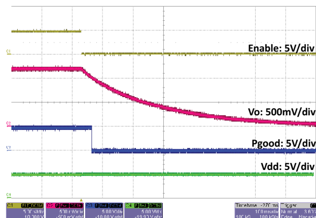
Fig. 32 - SiC451 Shut down with EN, t = 100\text{ ms/div}
