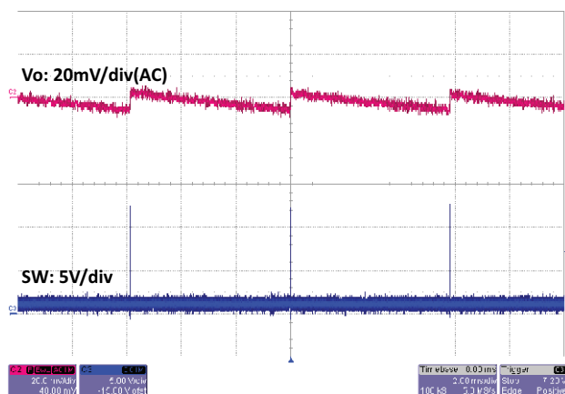
Fig. 42 - SiC451 Output Ripple, 0.01 A, t = 2\text{ ms/div} DCM Mode
