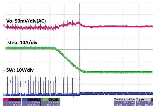
Fig. 58 - SiC450 Load Step, 20 A to 0 A, 1 A/ \mu\text{s} , t = 10\text{ }\mu\text{s/div} Skip Mode Enabled
