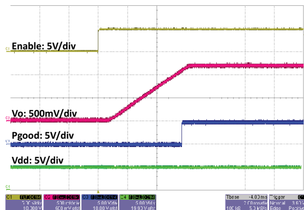
Fig. 31 - SiC451 Startup with EN, t = 2\text{ ms/div}
