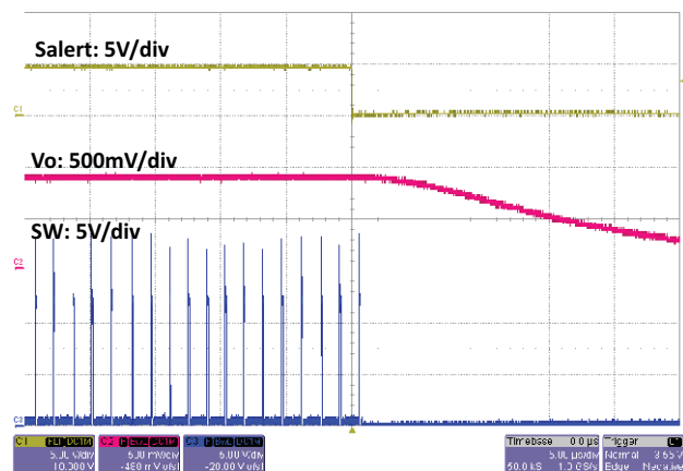
Fig. 52 - SiC450 Output Undervoltage Protection Behavior, t = 5\text{ }\mu\text{s/div}
