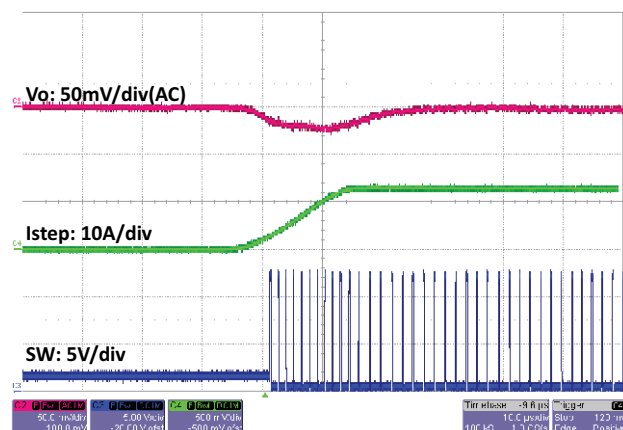
Fig. 39 - SiC451 Load Step, 0 A to 12.5 A, 1 A/μs, t = 10 μs/div Skip Mode Enabled
