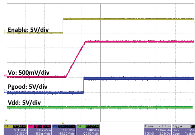
Fig. 49 - SiC450 Startup with EN, t = 5\text{ ms/div}
