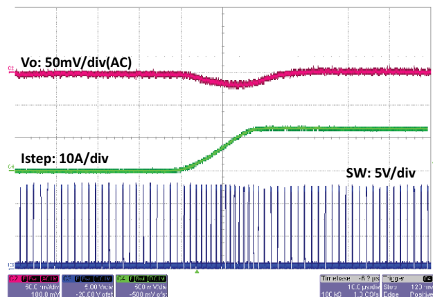
Fig. 37 - SiC451 Load Step, 0 A to 12.5 A, 1 A/μs, t = 10 μs/div
