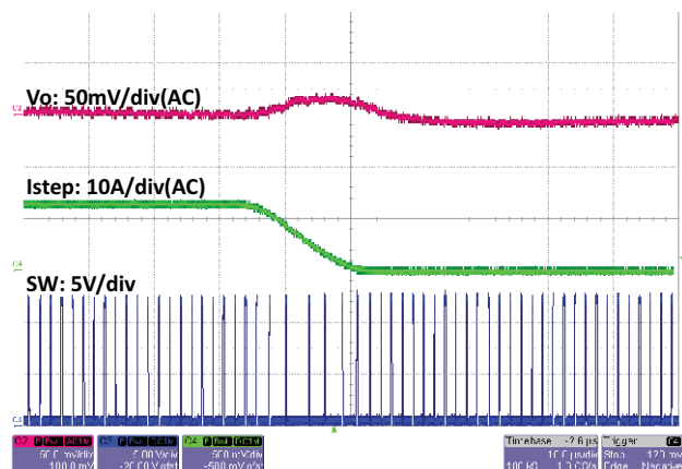
Fig. 36 - SiC451 Load Step, 25 A to 12.5 A, 1 A/μs, t = 10 μs/div
