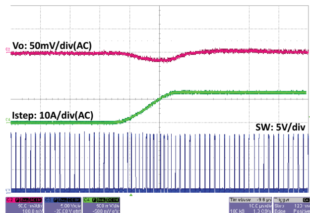
Fig. 35 - SiC451 Load Step, 12.5 A to 25 A, 10 A/μs, t = 10 μs/div
