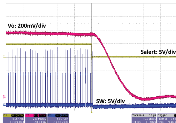
Fig. 16 - SiC453 UVP
