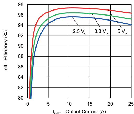
Fig. 46 - SiC451 Efficiency Curve
