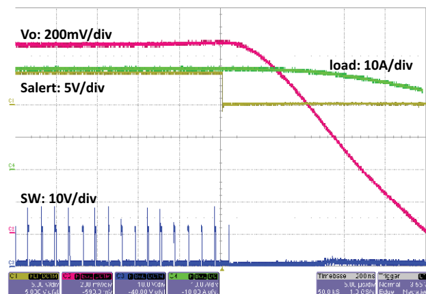
Fig. 33 - SiC451 OCP
