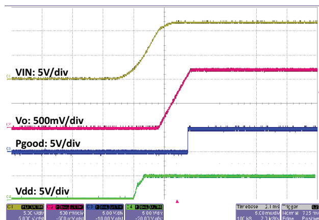
Fig. 47 - SiC450 Startup with V_{IN} , t = 5\text{ ms/div}
