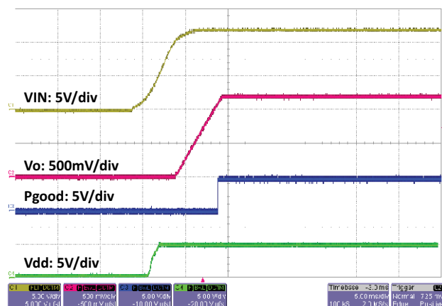
Fig. 29 - SiC451 Startup with V_{IN} , t = 5\text{ ms/div}
