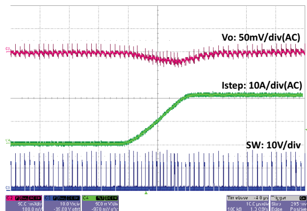
Fig. 53 - SiC450 Load Step, 20 A to 40 A, 1 A/ \mu\text{s} , t = 10\text{ }\mu\text{s/div}
