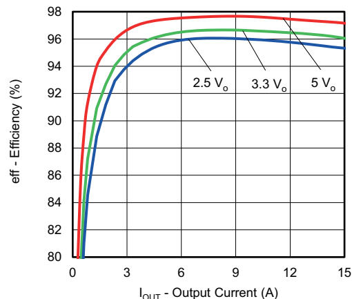
Fig. 28 - SiC453 Efficiency Curve
