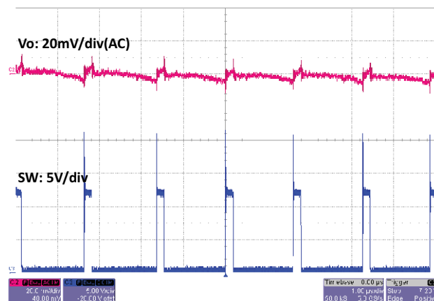
Fig. 44 - SiC451 Output Ripple, 25 A, t = 1\text{ }\mu\text{s/div} Forced Continuous Conduction Mode
