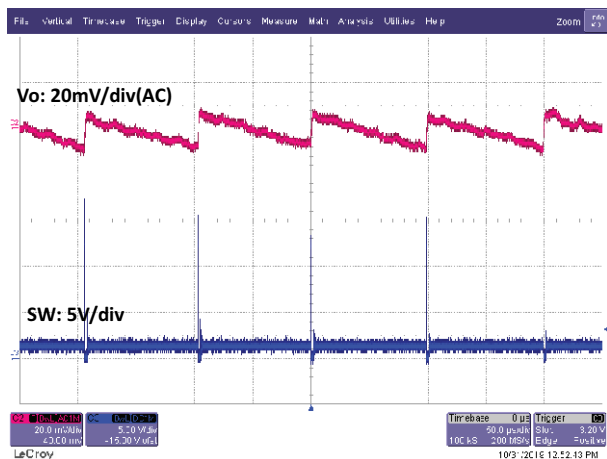
Fig. 60 - SiC450 Output Ripple, 0.01 A, t = 50\text{ }\mu\text{s/div} DCM Mode
