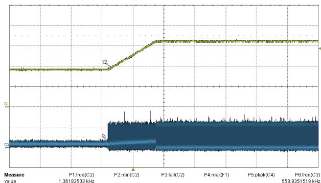
Fig. 8 - Pre-Bias Start-Up
