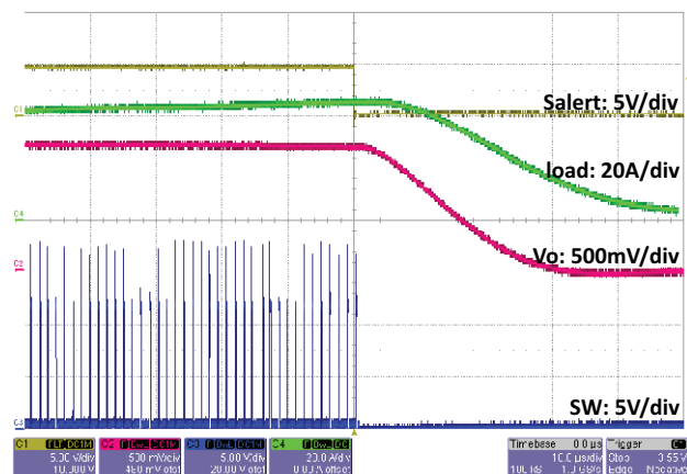
Fig. 51 - SiC450 Overcurrent Protection Behavior, t = 10\text{ }\mu\text{s}
