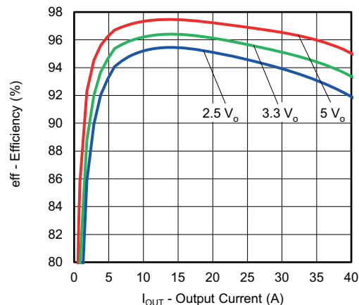
Fig. 64 - SiC450 Efficiency Curve
