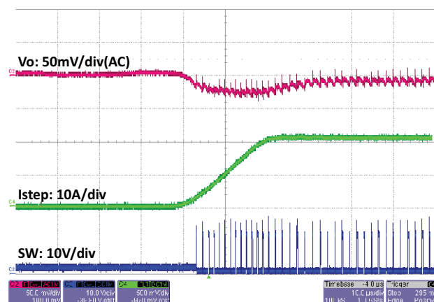
Fig. 57 - SiC450 Load Step, 0 A to 20 A, 1 A/ \mu\text{s} , t = 10\text{ }\mu\text{s/div} Skip Mode Enabled
