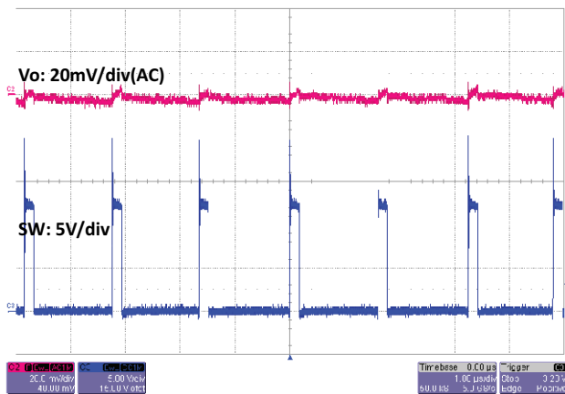
Fig. 61 - SiC450 Output Ripple, 20 A, t = 1\text{ }\mu\text{s/div} Forced Continuous Conduction Mode
