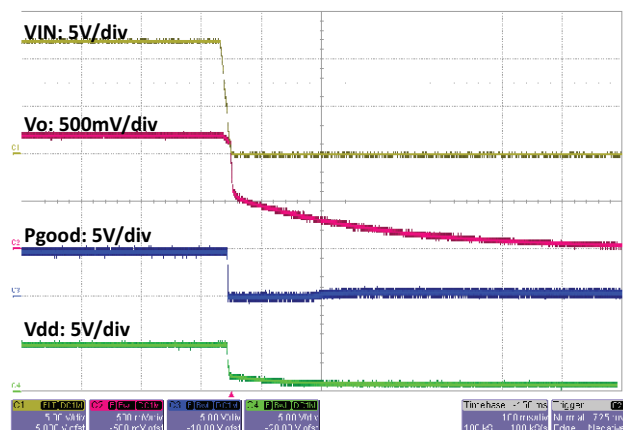
Fig. 30 - SiC451 Shut Down with V_{IN} , t = 100\text{ ms/div}
