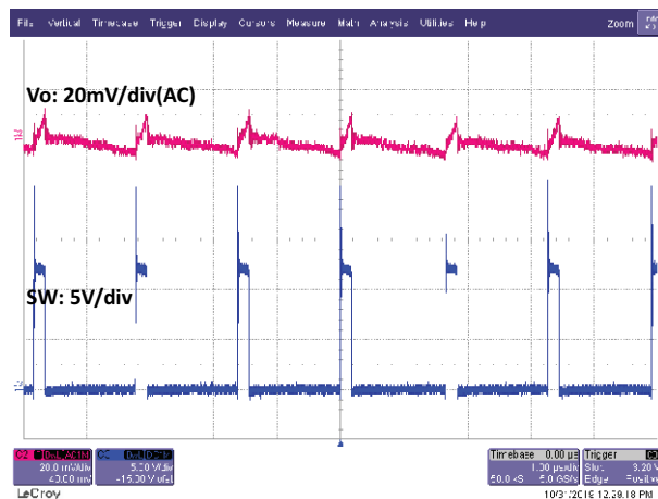
Fig. 62 - SiC450 Output Ripple, 40 A, t = 1\text{ }\mu\text{s/div} Forced Continuous Conduction Mode
