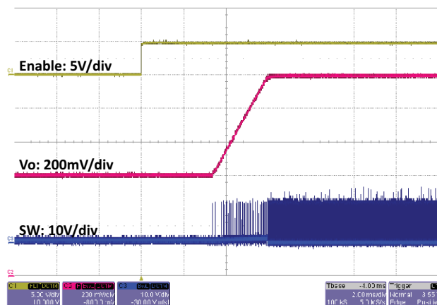
Fig. 63 - SiC450 Prebias Startup
