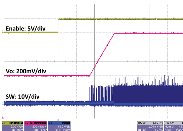
Fig. 45 - SiC451 Prebias Startup
