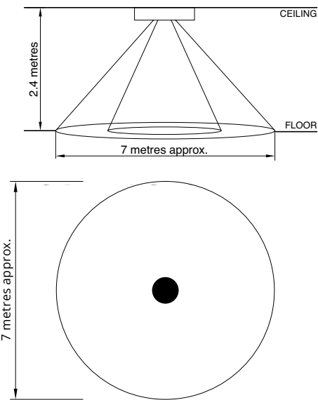
Ceiling mount PIR sensor detection diagram
