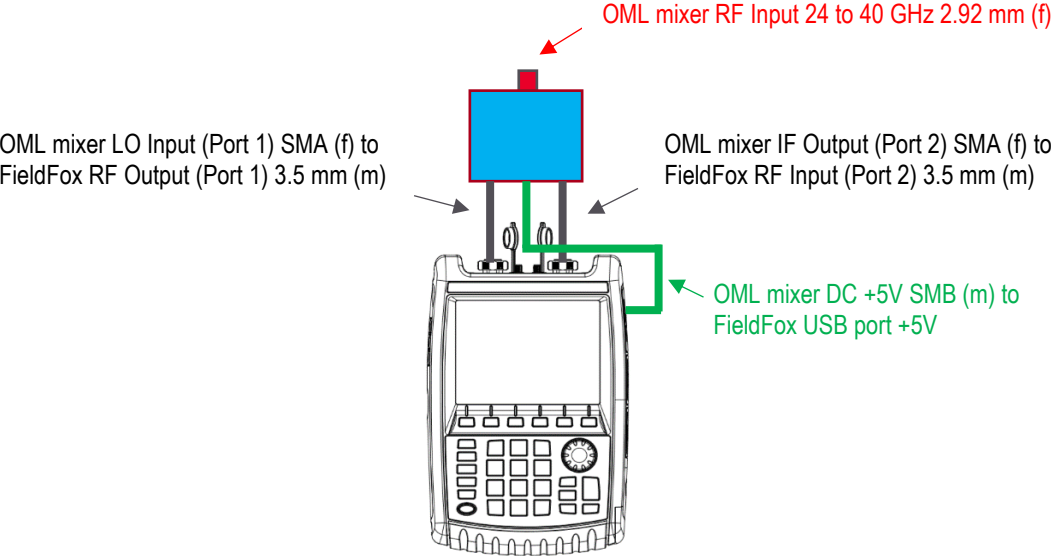
Figure 1 – OML external mixer diagram
