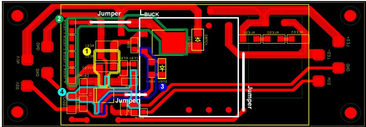
Figure 15. Layout Guidance
