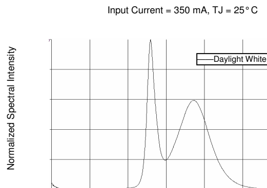
Wavelength Characteristics
