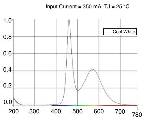
Wavelength Characteristics
