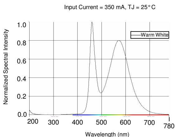
Wavelength Characteristics
