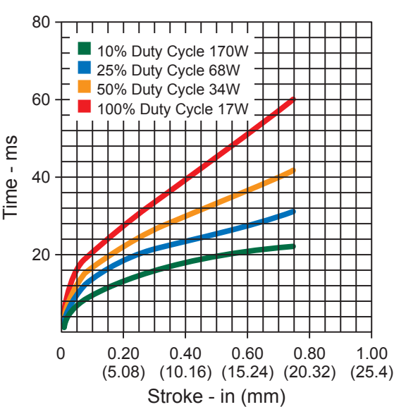
Typical Speed @ No Load, 20°C
