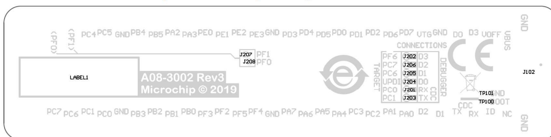
Figure 7-3. AVR128DA48 Curiosity Nano Assembly Drawing Bottom
