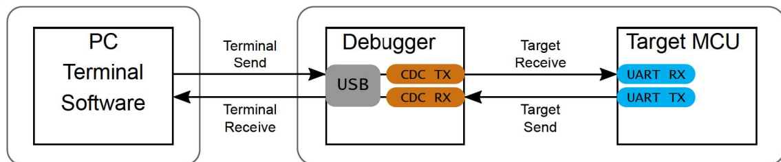
Figure 3-1. CDC Connection
