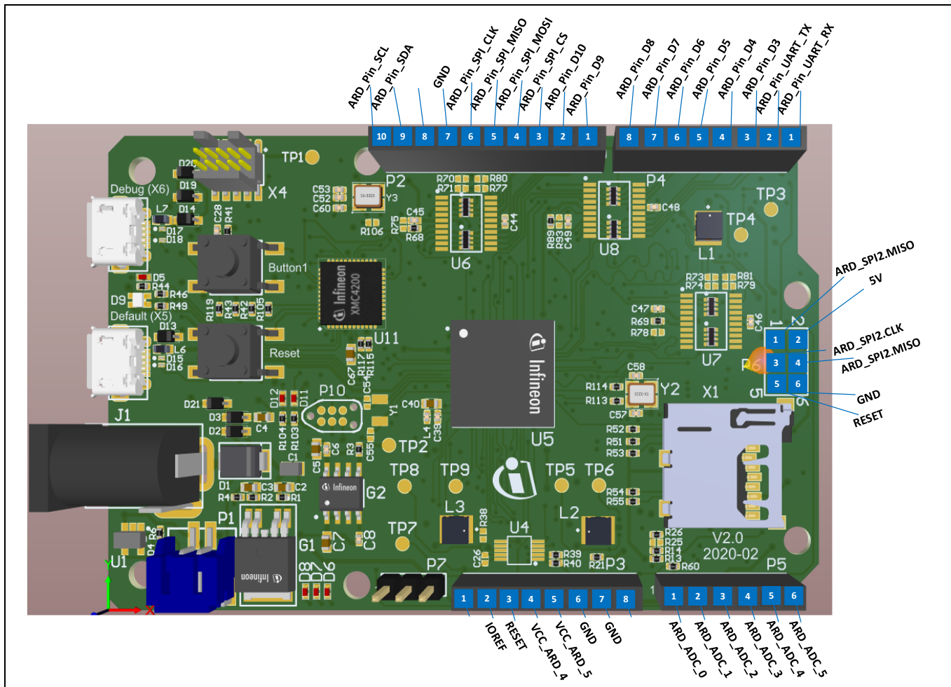
Figure 16 External headers – P2, P3, P4, P5 and P6
