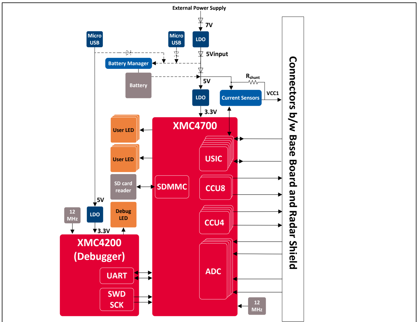
Figure 2 Block diagram – Radar Baseboard XMC4700
