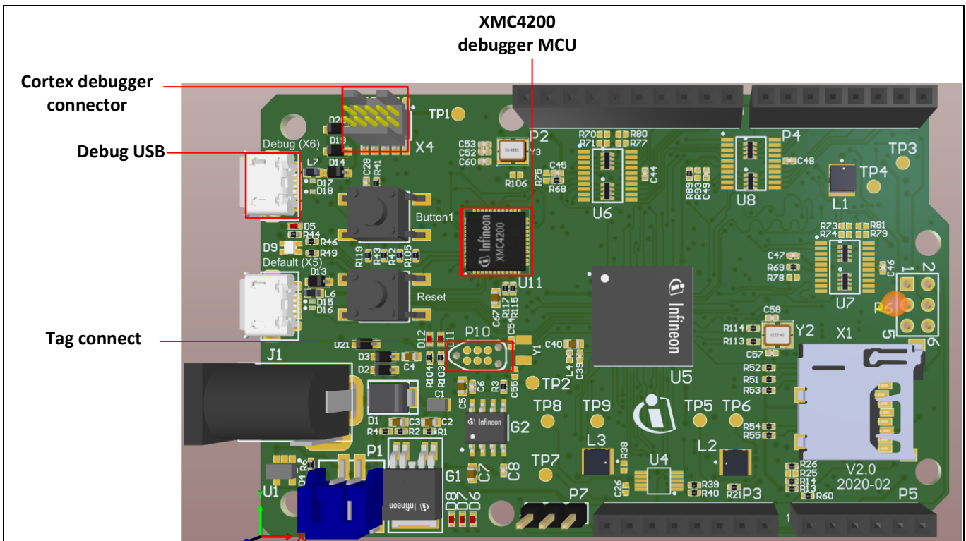
Figure 19 V2.0 Debugger components – For debugging and flashing, the USB cable has to be simply connected to the “Debug USB” port. Header settings are no longer needed.
