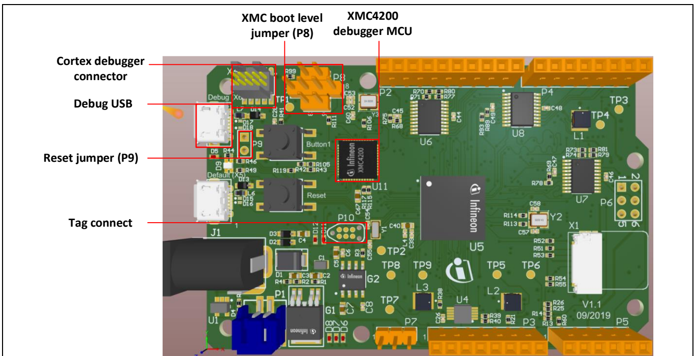
Figure 17 V1.1 Debugger components
