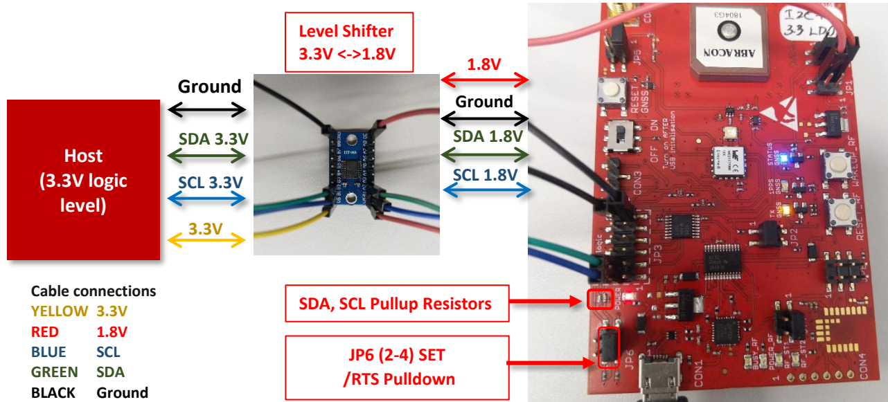
Figure 16: Elara-II- GNSS evaluation board connection to 3.3V Host
