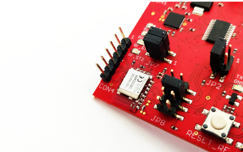
Figure 2: 2613029237011 - detail of the Thyone-I RF interface
