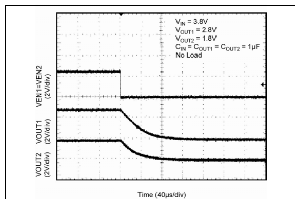
FIGURE 2-16: Turn-Off Time MIC5381 (Auto-Discharge).
