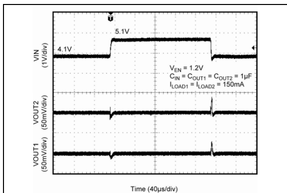
FIGURE 2-13: Line Transient.
