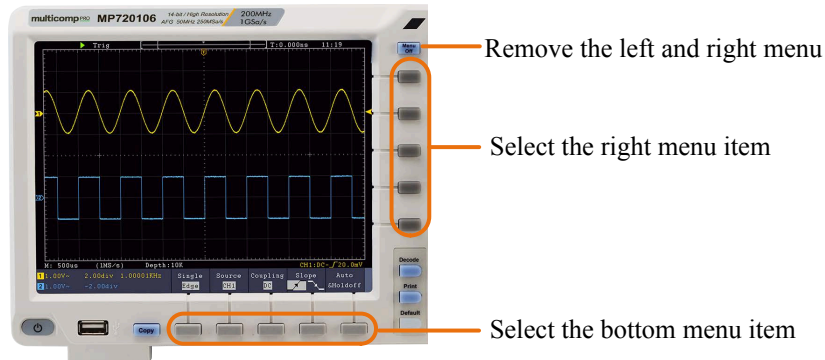
Figure 3-2 Menu Buttons
