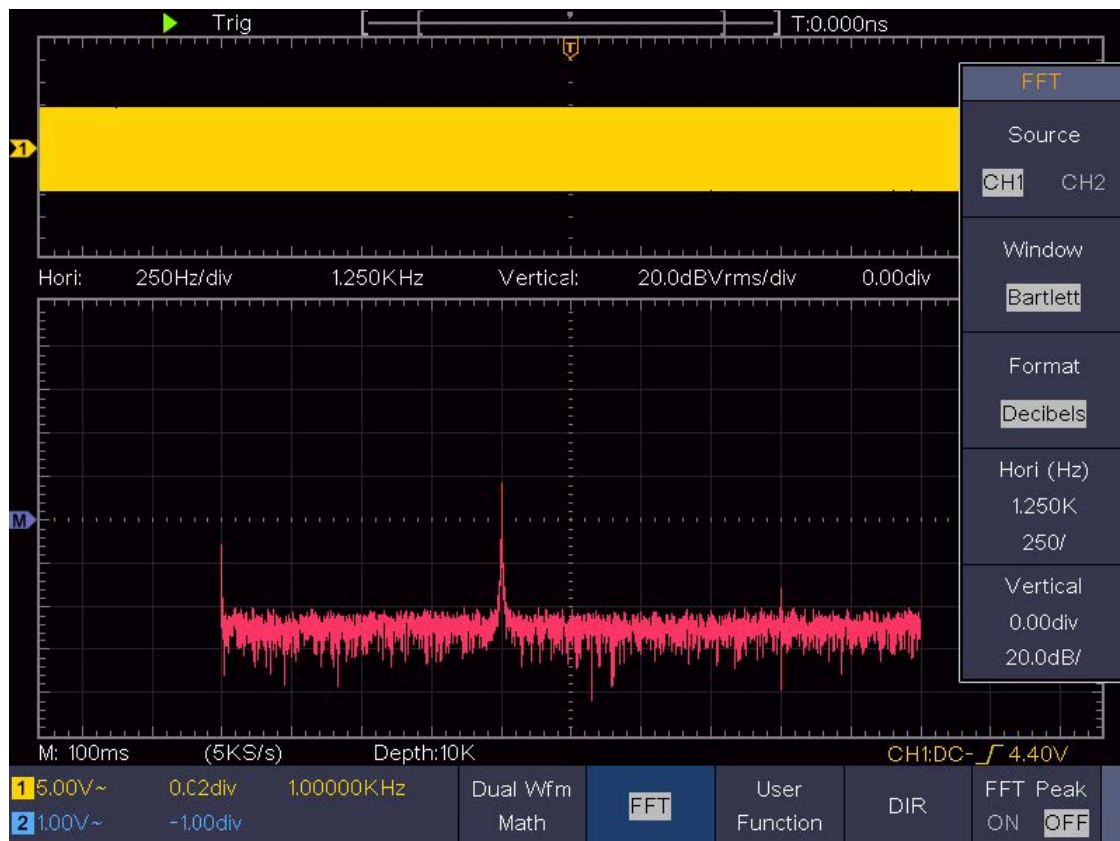
Figure 4-6 Bartlett window
