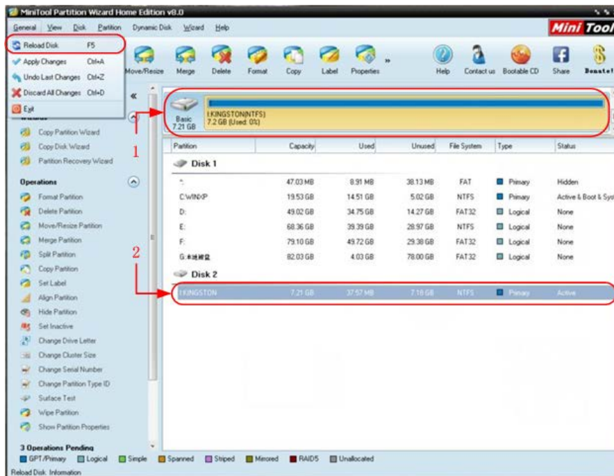
Figure 4-13: Reload Disk
