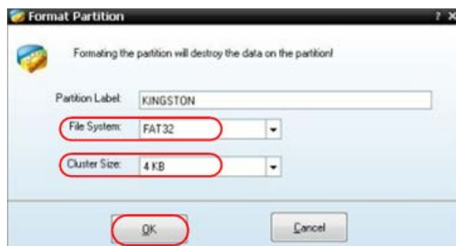
Figure 4-15: Format setting
