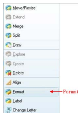
Figure 4-14: Choose format
