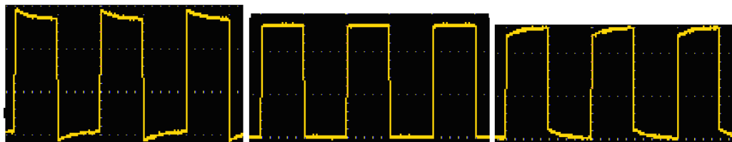
Overcompensated Compensated correctly Under compensated Figure 3-7 Displayed Waveforms of the Probe Compensation
