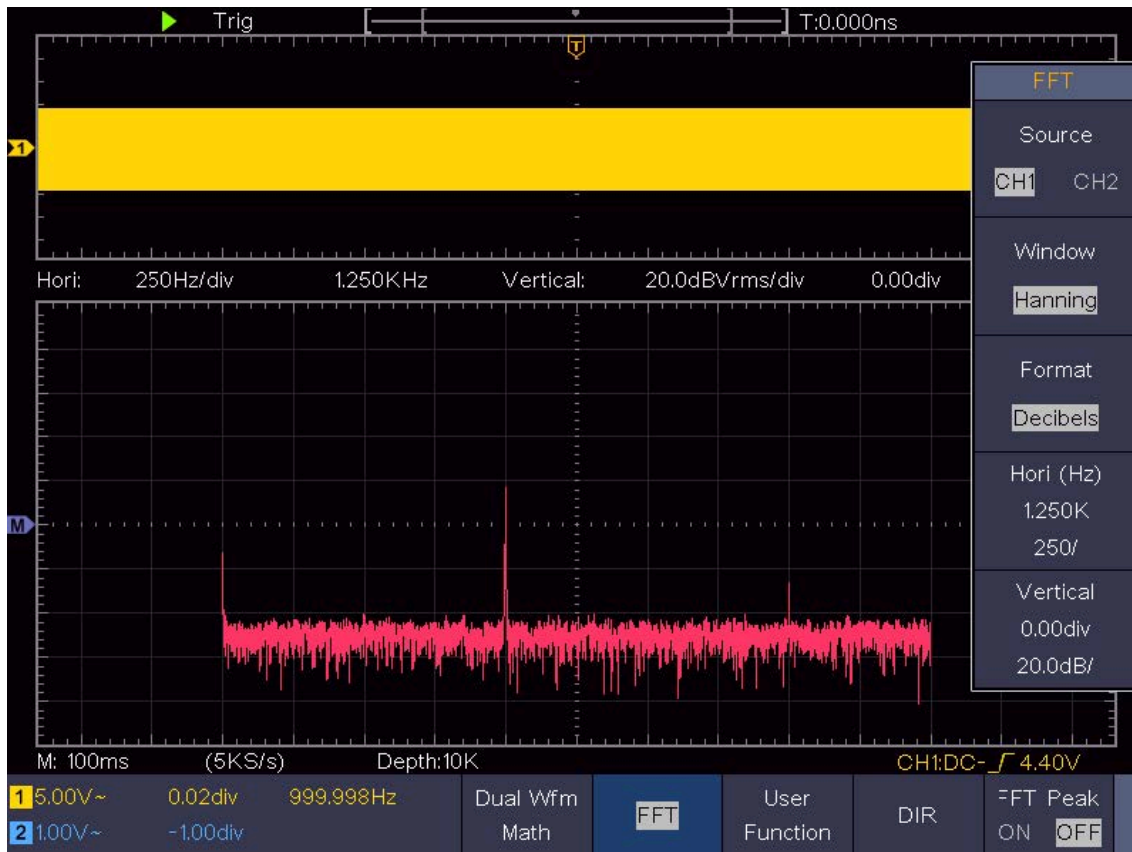
Figure 4-4 Hanning window
