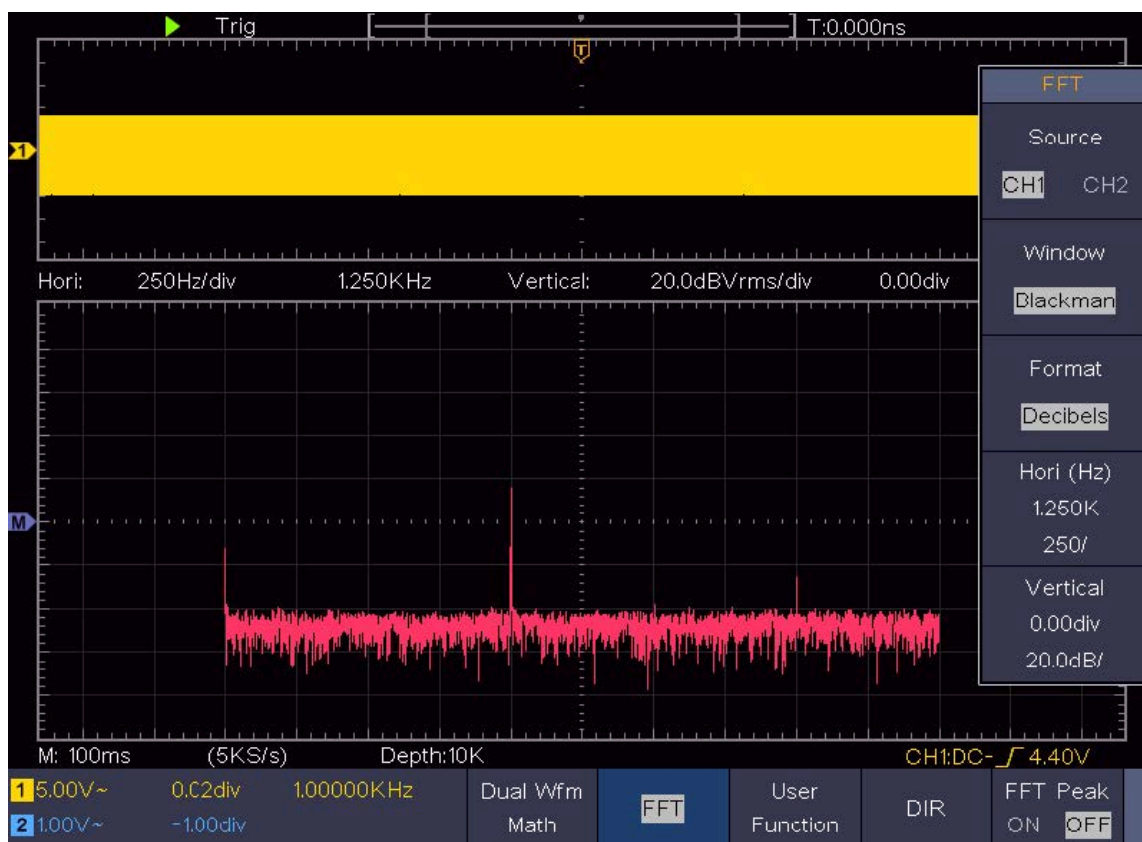
Figure 4-3 Blackman window
