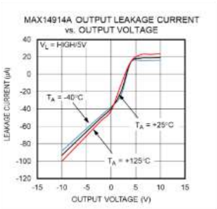
Figure 6. MAX14914A output leakage ( V_L = \text{HIGH}/5V ).
