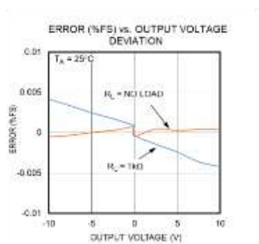
Figure 12. Error (%FSR) for analog voltage output at different loads with calibration performed with no load.
