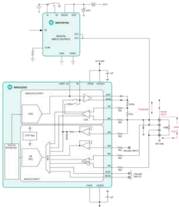
Figure 18. Analog input current-mode configuration.
