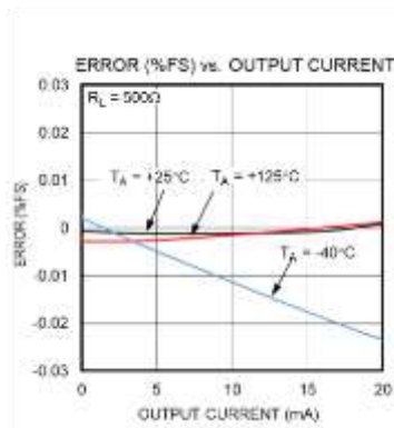
Figure 17. Error (%FSR) for analog current output at different temperatures with a 500\Omega load and positive loop currents.
