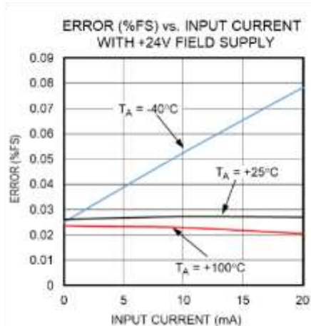
Figure 21. Error (%FSR) performance at different temperatures.
