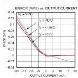
Figure 15. Total error (%FSR) vs. \pm 20\text{mA} output current.
