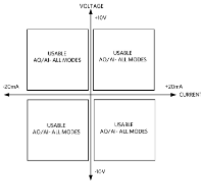
Figure 3. Four-quadrant voltage/current application.
