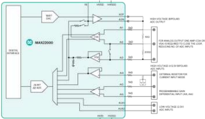
Figure 2. The MAX22000 as an analog IO.
