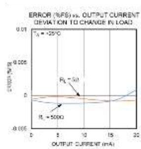
Figure 16. Error (%FSR) for analog current output comparison with different loads (calibration performed with a 5\Omega load).
