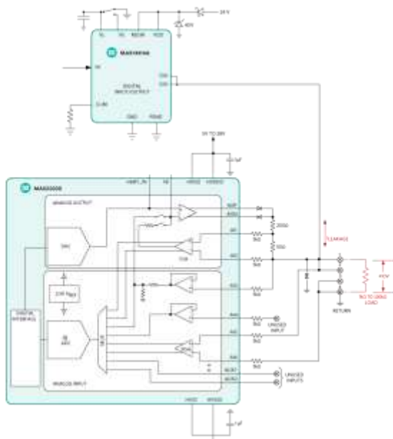
Figure 11. Analog output voltage mode configuration.
