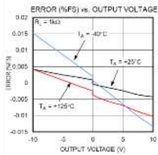
Figure 13. Error (%FSR) for analog voltage output at different temperatures with 1kΩ load.
