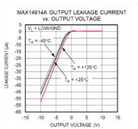
Figure 7. MAX14914A output leakage ( V_L = \text{LOW}/\text{GND} ).
