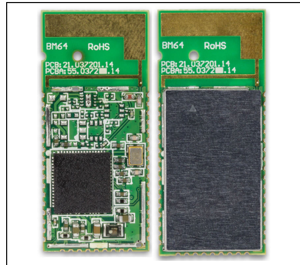
FIGURE 2: BM64 MODULE
