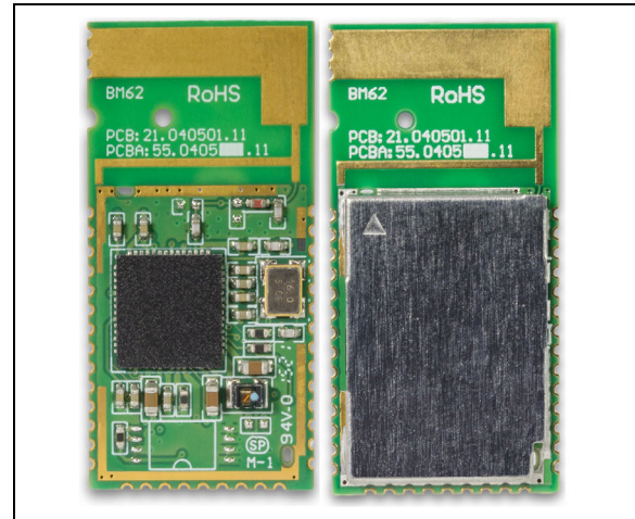
FIGURE 1: BM62 MODULE
