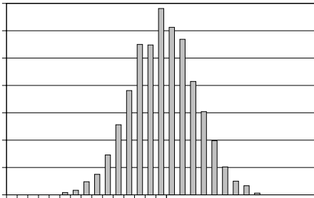
FIGURE 2-1: Input Offset Voltage Histogram at V_{CM} = V_{SS} .
