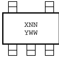
5-Lead SOT-23 (MCP6541)
