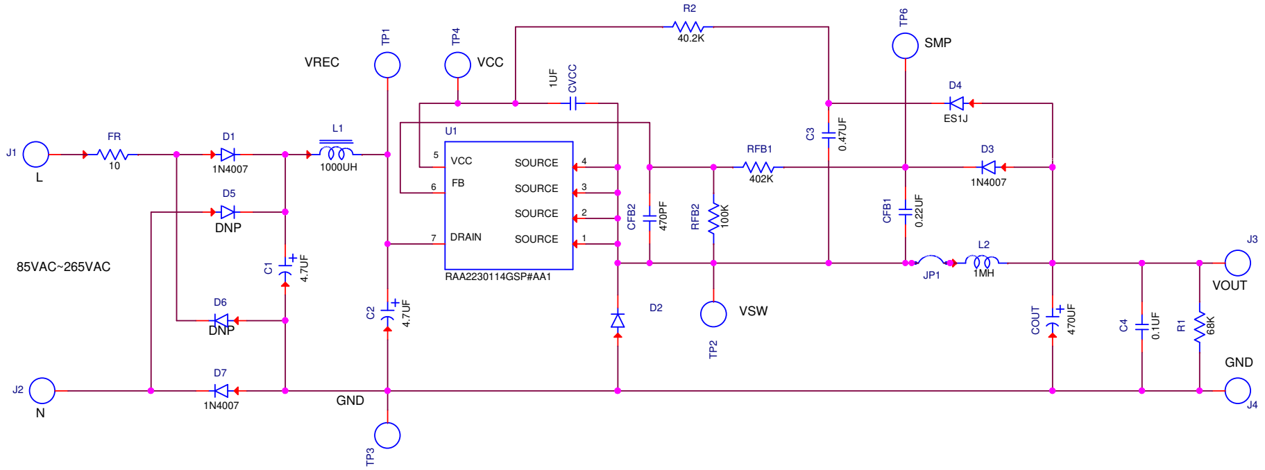
Figure 4. RTKA223011DE0020BU Schematic
