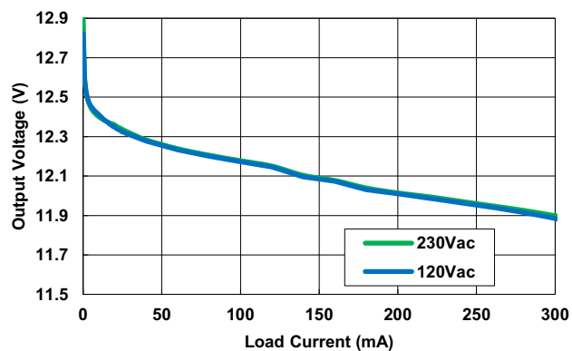
Figure 8. Load Regulation
