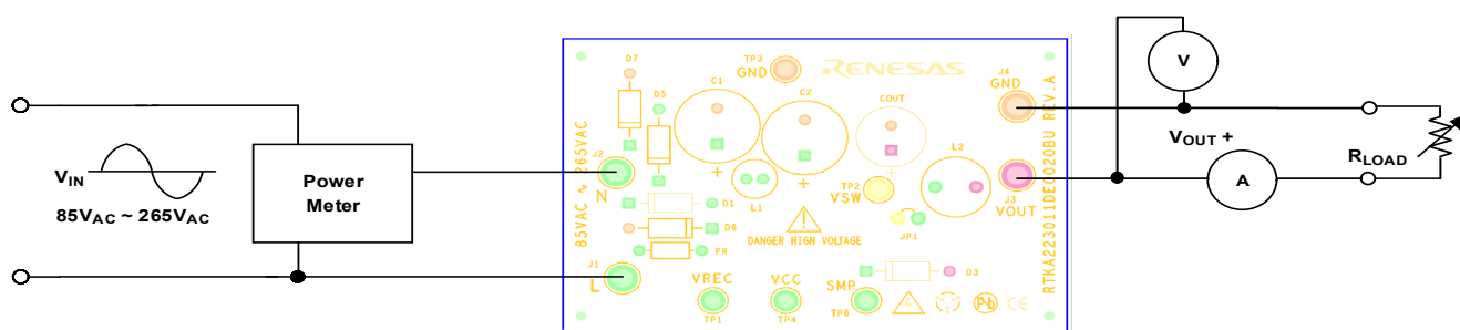
Figure 1. RTKA223011DE0020BU Connection Diagram
