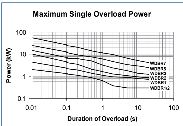
Mounted on a 0.53^{\circ}\text{C}/\text{W} heatsink with 5m/s forced air cooling, air temperature 25^{\circ}\text{C} . \Delta R \leq 5\% .
