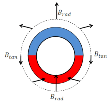
Figure 20: Side-Shaft Field
