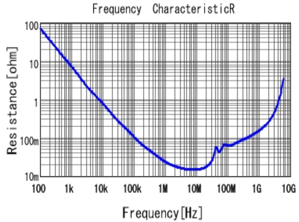
■ GRM188R72A104KA35 R DCOV, 25degC
