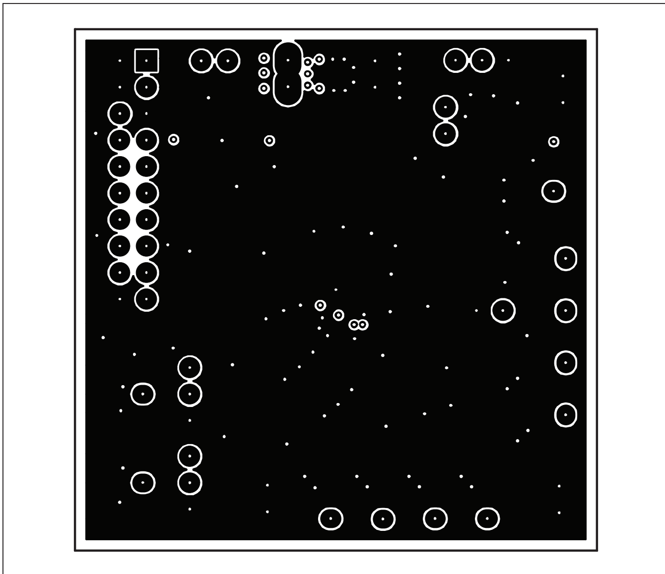
MAX20480 EV Kit Component Placement Guide – Internal 2
