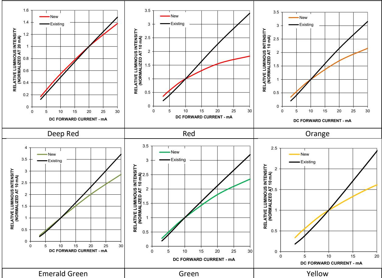
Figure 4: Relative Intensity vs Forward Current
