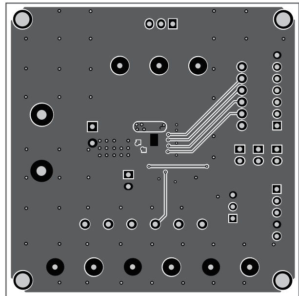
Figure 5: Bottom Layer
