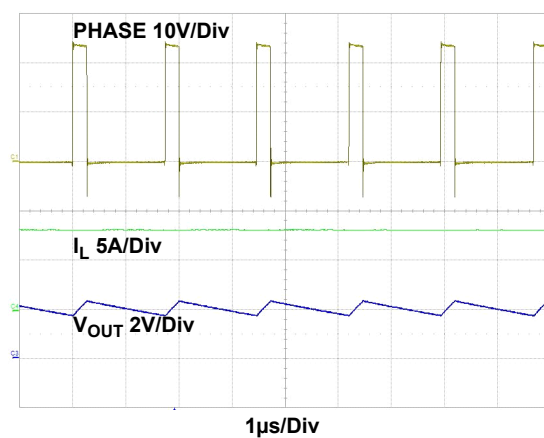
Figure 12. Steady-State Operation I_{OUT} = 5A
