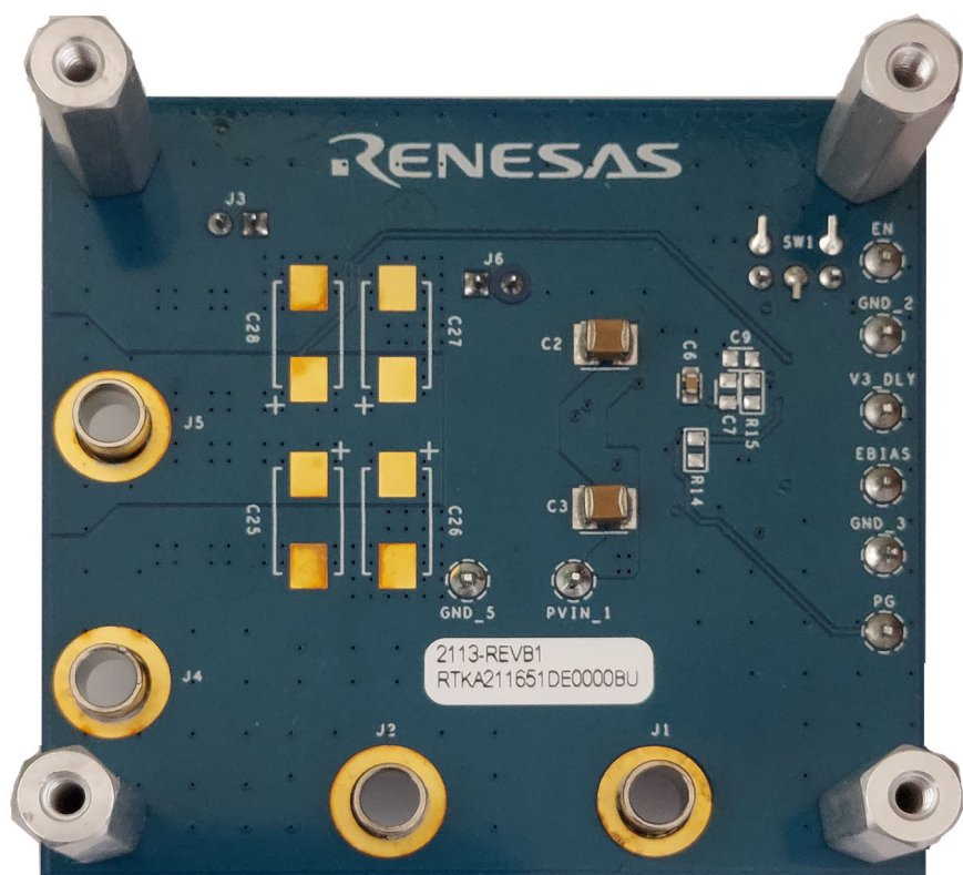
Figure 3. RTKA211651DE0000BU Evaluation Board (Bottom)
