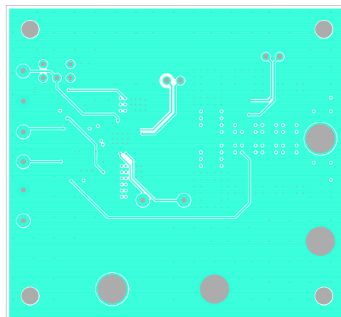
Figure 8. Layer 3
