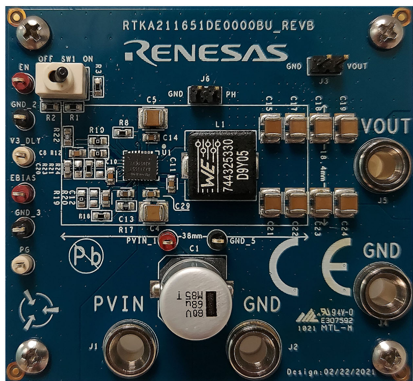
Figure 2. RTKA211651DE0000BU Evaluation Board (Top)
