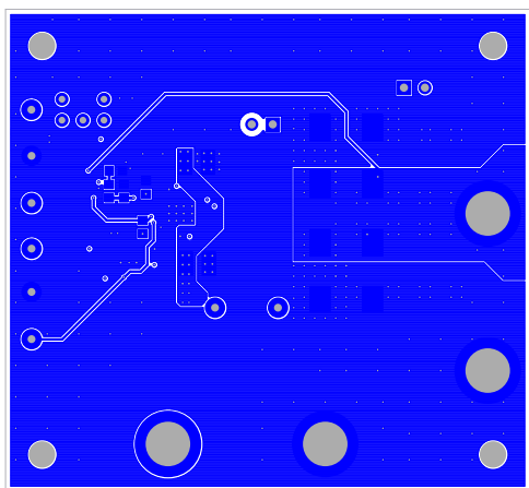
Figure 9. Bottom Layer
