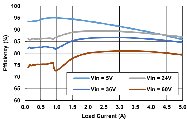
Figure 11. Efficiency vs Load Current ( V_{OUT} = 3.3V )
