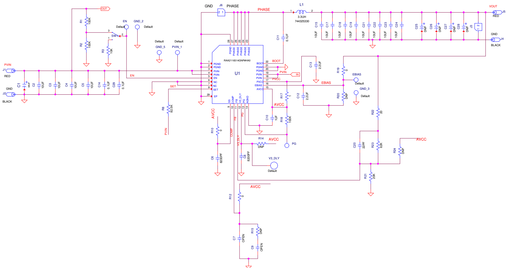
Figure 4. RTKA211651DE0000BU Schematic
