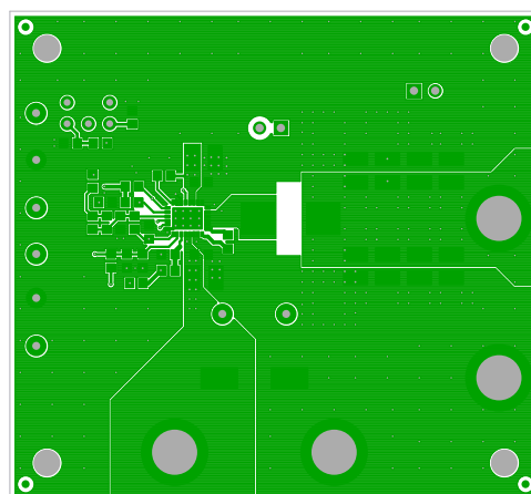
Figure 6. Top Layer
