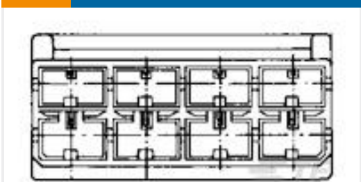
TE Part #926646-8 PL 250 8P HOUSING PA6.6 ZYTEL 101 WHITE
