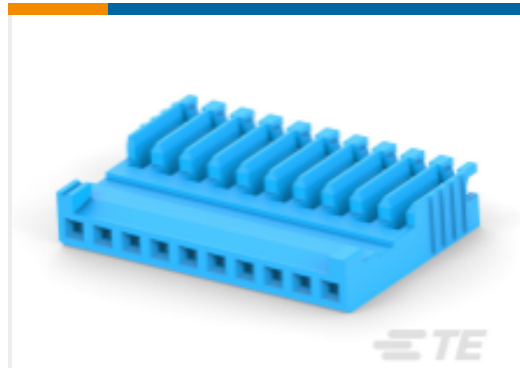
TE Part #1-281786-2 HE13/HE14 IDC Receptacle, SRST, AWG24-2
