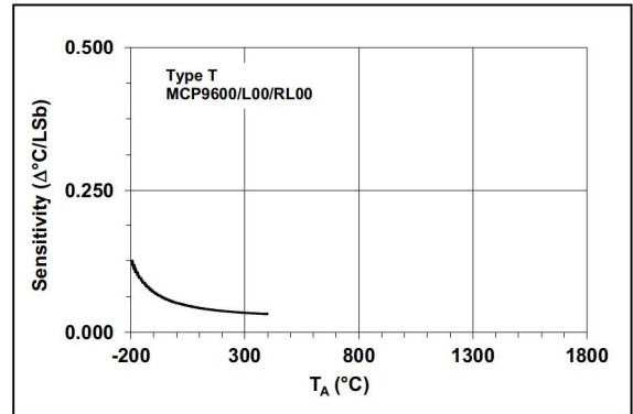
FIGURE 2-16: Temperature Sensitivity with 18-Bit Resolution, Type T.
