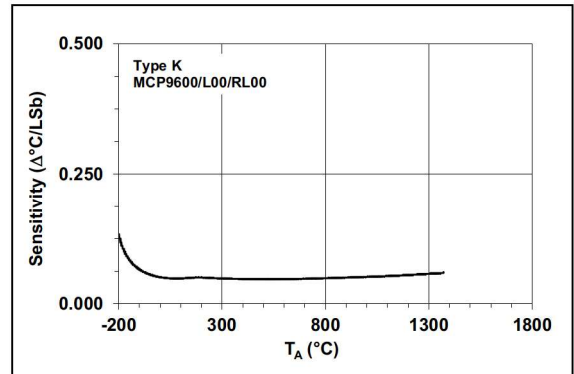
FIGURE 2-4: Temperature Sensitivity with 18-Bit Resolution, Type K.
