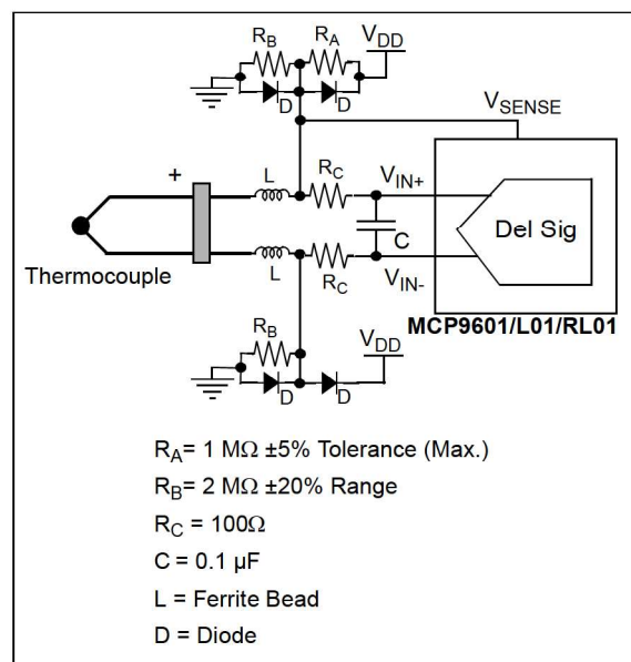
FIGURE 6-12: Adding Ferrite Beads (MCP9601/L01/RL01).
