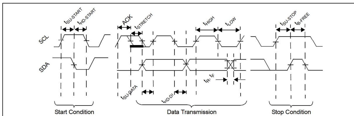
FIGURE 1-2: Timing Diagram.
