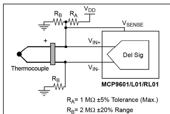
FIGURE 6-7: Adding Open-Circuit Detection Resistors (MCP9601/L01/RL01).
