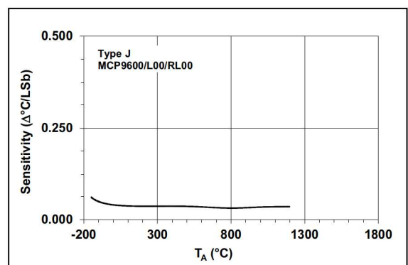
FIGURE 2-5: Temperature Sensitivity with 18-Bit Resolution, Type J.
