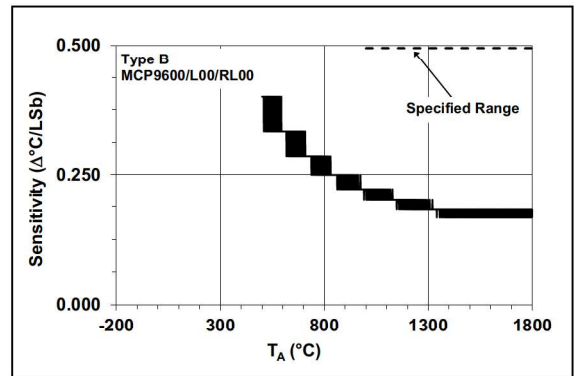
FIGURE 2-17: Temperature Sensitivity with 18-Bit Resolution, Type B.
