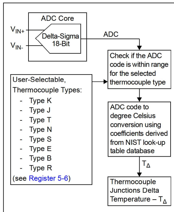
FIGURE 5-3: Thermocouple Hot-Junction Register ( T_{\Delta} ) Block Diagram.
