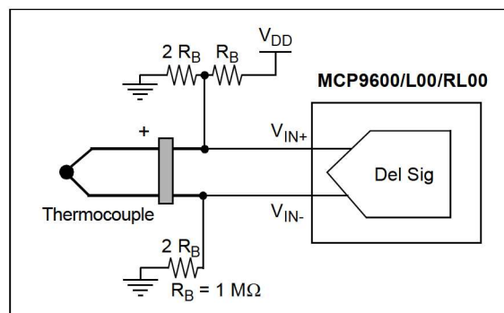
FIGURE 6-6: Adding Open-Circuit Detection Resistors (MCP9600/L00/RL00).
