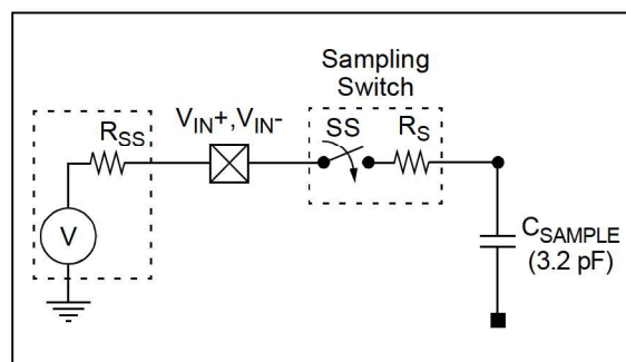
FIGURE 6-5: Thermocouple Input Stage.
