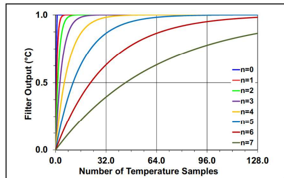
FIGURE 5-6: Filter Step Response.
