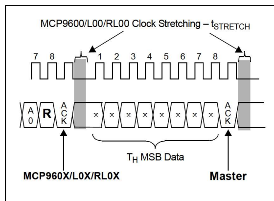
FIGURE 4-2: Clock Stretching.
