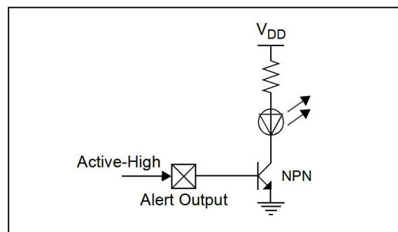
FIGURE 6-3: Alert Output Buffer for LED Indicator.
