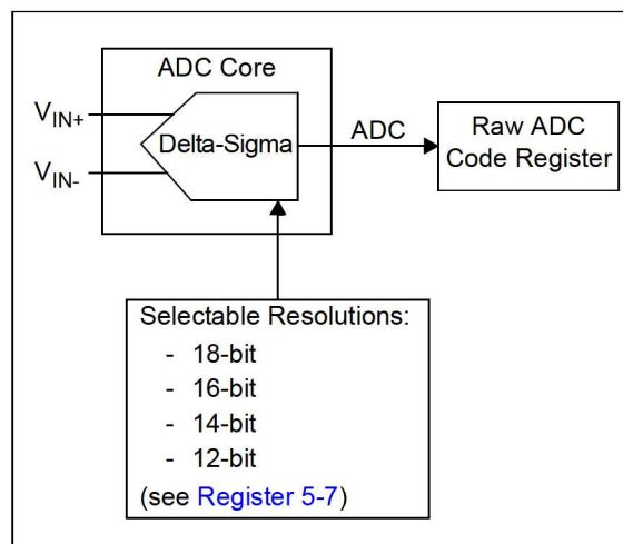
FIGURE 5-5: Delta-Sigma Analog-to-Digital Converter, ADC Core Block Diagram.
