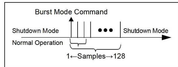
FIGURE 5-7: Burst Mode Operation.
