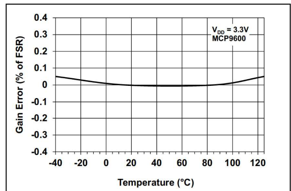
FIGURE 2-18: Full-Scale Gain Error.
