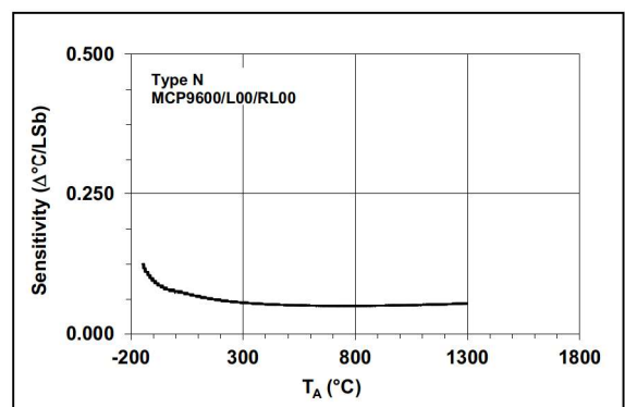
FIGURE 2-6: Temperature Sensitivity with 18-Bit Resolution, Type N.
