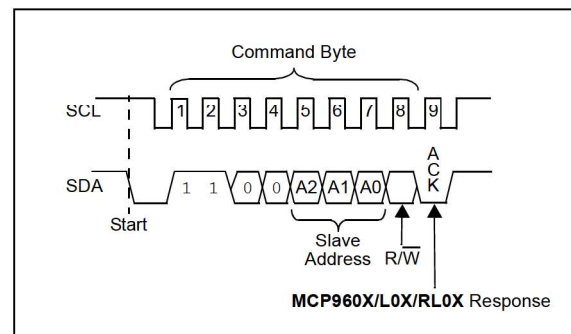
FIGURE 4-1: Device Addressing.
