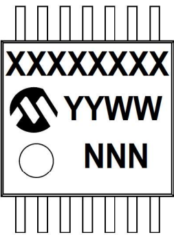
14-Lead TSSOP (MCP6479)
