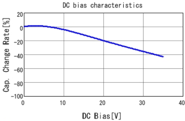
■ KCM55WR7YA336MH01 C-DC bias capchange, 25.0degC, AC0.
