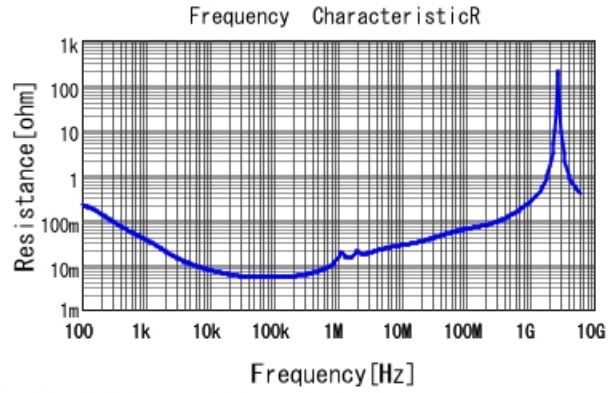
■ KCM55WR7YA336MH01 R DCOV, 25degC
