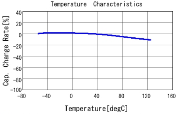
■ KCM55WR7YA336MH01 C-Temp. capchange, DCOV, ACO. 5Vrms
