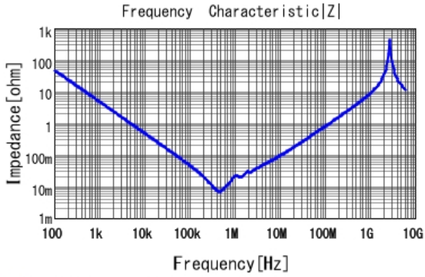
■ KCM55WR7YA336MH01 |Z| DCOV, 25degC
