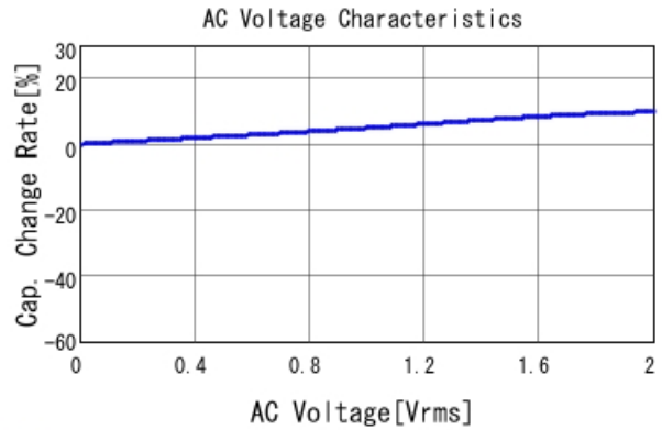
■ KCM55WR7YA336MH01 C-AC Voltage capchange, DCOV, 25.0d
