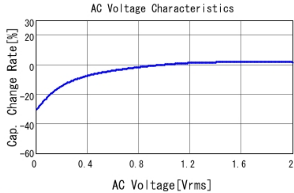
■ GRM188R61E106KA73 C-AC Voltage capchange, DCOV, 25.0d
