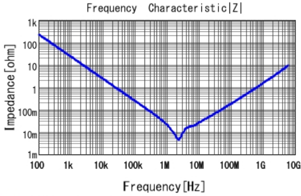
■ GRM188R61E106KA73 |Z| DCOV, 25degC
