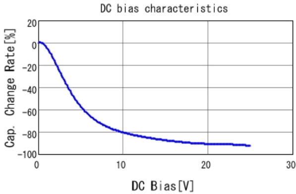
■ GRM188R61E106KA73 C-DC bias capchange, 25.0degC, AC1V
