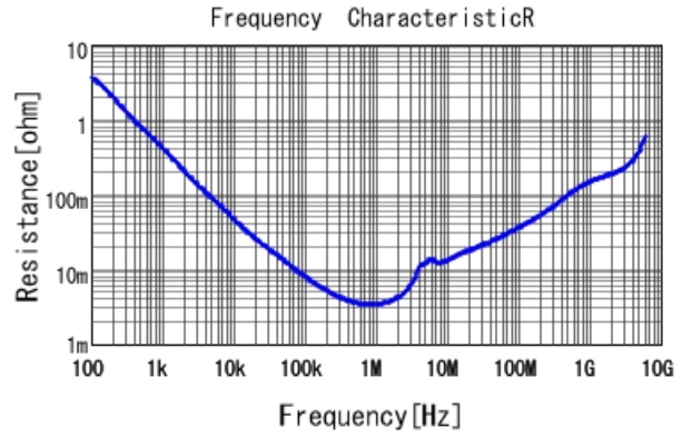
■ GRM188R61E106KA73 R DCOV, 25degC
