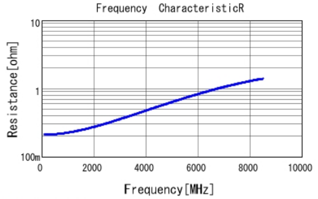
■ GRM0335C2A5R1CA01 R DCOV, 25degC
