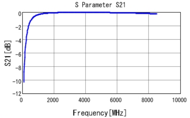
■ GRM0335C2A5R1CA01 S21 DCOV, 25degC
