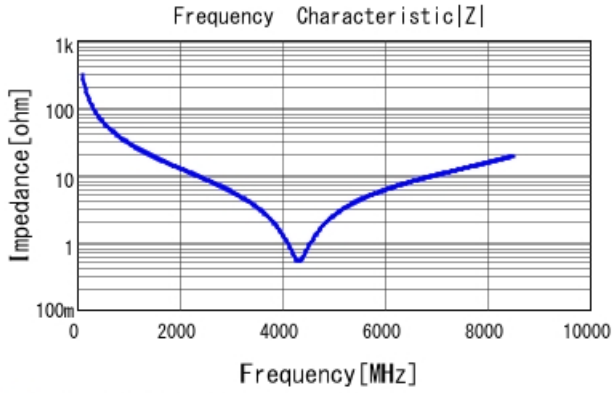
■ GRM0335C2A5R1CA01 |Z| DCOV, 25degC
